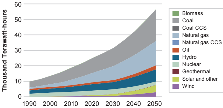
Figure 2.9: Global electric generation by fuel under the baseline scenario from 1990 to 2050, in thousands of terawatt hours (TWh)
