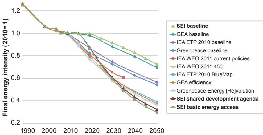
Figure 2.20: Comparison of global final energy intensity in SEI and selected scenarios
