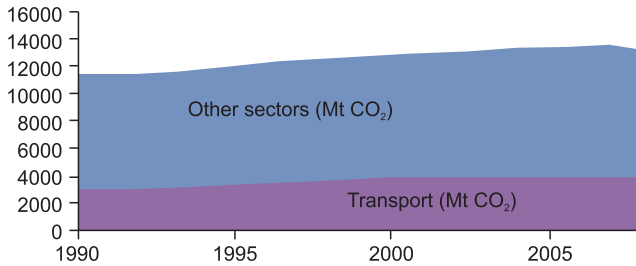
Figure 3.3: CO 2 emissions in megatonnes (Mt) from transport in 2008 (top) and change in CO 2 emissions from transport from 1990 to 2008, compared with other sectors (bottom)
