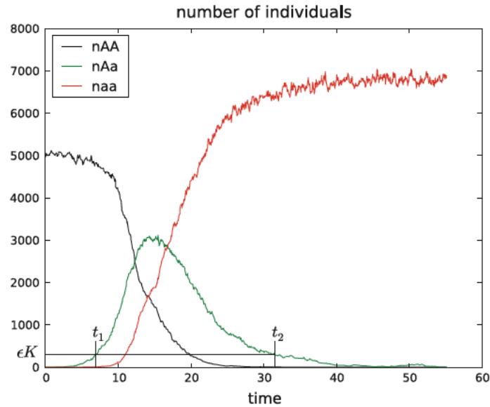
Fig. 1 Simulation of the three phases of mutant invasion
