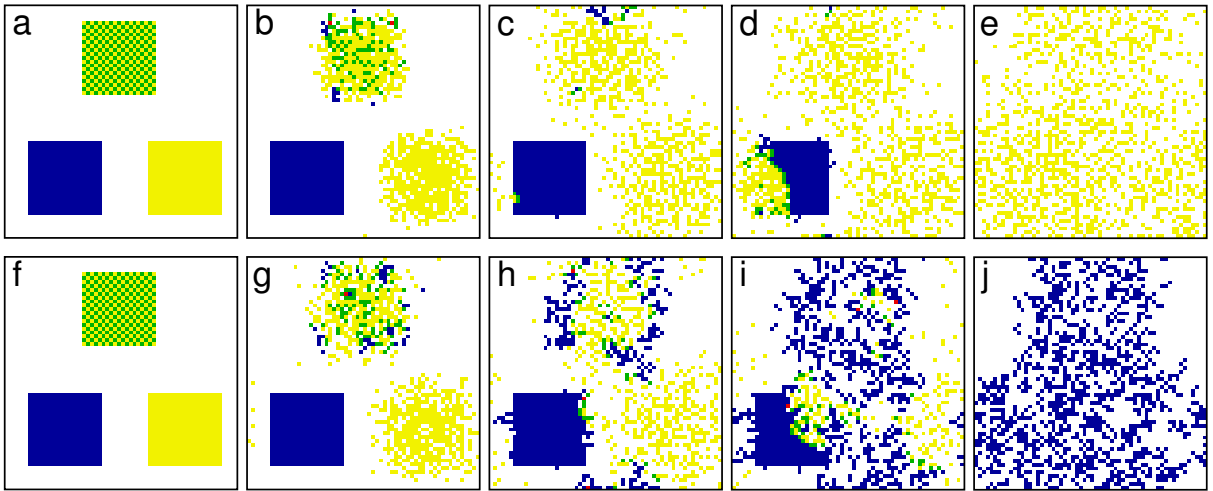
FIG. 4: (Color online) Pattern formation as observed from a prepared initial at \alpha = 0.8 . The risk probability parameter is \beta = 0.6 [upper row from (a) to (e)] and \beta = 0.1 [bottom row from (f) to (j)]. Cooperators whose focal group succeeds (fails) to reach the collective target are denoted blue (green). Similarly, defectors whose focal group succeeds (fails) are denoted red (yellow). White marks empty sites. Other parameters are: \rho = 0.30 , c/b = 0.5 and L = 60 . Monte Carlo steps are t = 0, 3, 21, 40, 120 for panels (a) to (e), and t = 0, 8, 40, 85, 380 for panels (f) to (j), respectively.
