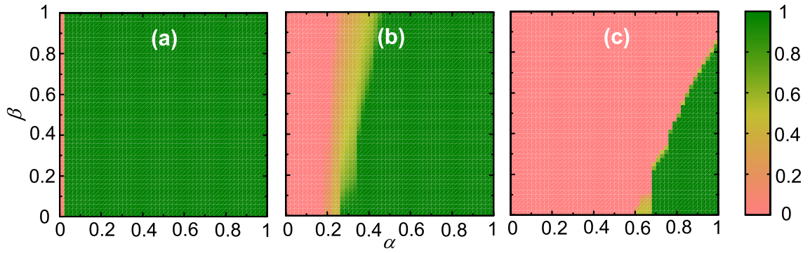
FIG. 2: (Color online) Fraction of cooperators in dependence on \alpha and \beta in a contour plot form for three different donation ratios: (a) c/b = 0.1 , (b) c/b = 0.3 and (c) c/b = 0.5 . In all three panels the density of players is \rho = 0.3 .
