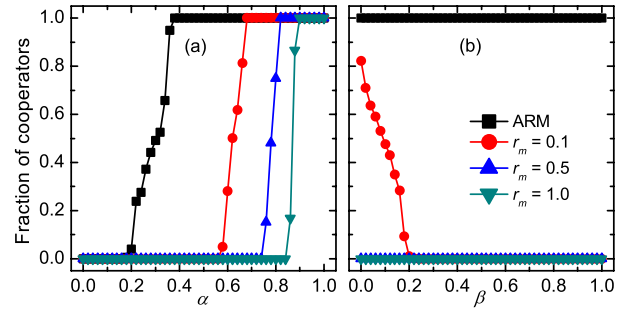
FIG. 7: (Color online) In panel (a) the fraction of cooperators is presented as a function of \alpha for a fixed value of \beta = 0.5 and different constant migration rates. In panel (b) the fraction of cooperators is presented as a function of \beta for a fixed value of \alpha = 0.5 and different constant migration rates. The population density is \rho = 0.3 and c/b = 0.3 . Also depicted in both panels are results obtained with adaptive risk-migration (ARM).
