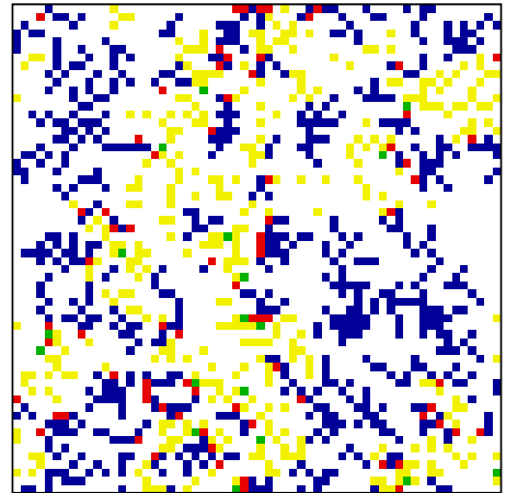
FIG. 5: (Color online) Representative snapshot of a stationary mixed phase, as obtained for \alpha = 0.4 , \beta = 0.9 , c/b = 0.3 and \rho = 0.30 . The color code is identical to the one used in Figs. 3 and 4.
