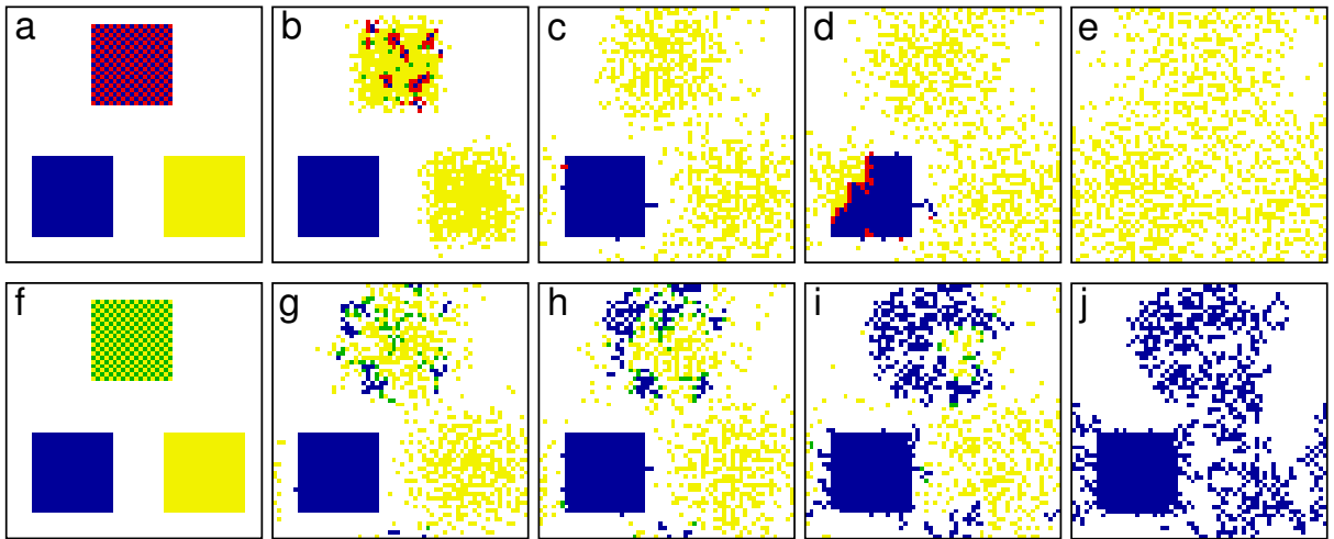
FIG. 3: (Color online) Pattern formation as observed from a prepared initial at \beta = 0.2 . The weighting factor related to collective threshold is \alpha = 0.2 [upper row from (a) to (e)] and \alpha = 0.9 [bottom row from (f) to (j)]. Cooperators whose focal group succeeds (fails) to reach the collective target are denoted blue (green). Similarly, defectors whose focal group succeeds (fails) are denoted red (yellow). White marks empty sites. Other parameters are: \rho = 0.30 , c/b = 0.5 and L = 60 . Monte Carlo steps are t = 0, 3, 25, 40, 90 for panels (a) to (e), and t = 0, 18, 30, 53, 465 for panels (f) to (j), respectively.
