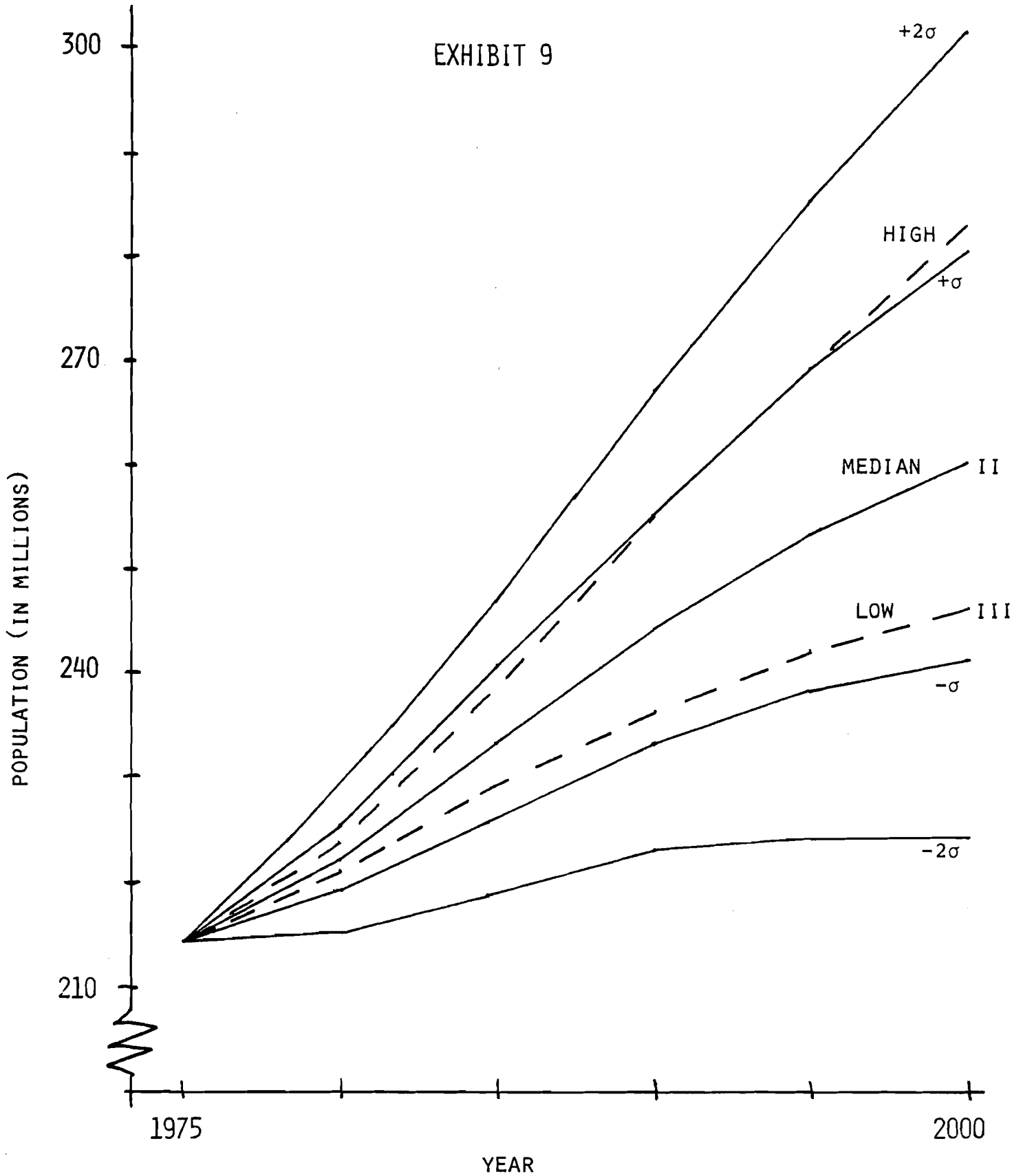
U.S. CENSUS PROJECTIONS (HIGH, MEDIAN, LOW) AND \sigma = .3 CONFIDENCE INTERVALS
