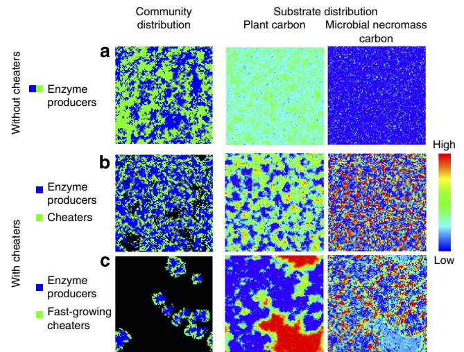
Figure 2 | Spatial distributions of microbes and substrate in litter decomposition. Distributions with and without microbial cheaters.
