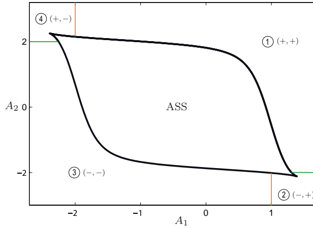
Figure 4: Region of Alternative Stable States (ASS) in the space of the appeals and signs of the feelings in regions ①, ②, ③, and ④ outside ASS. Parameters and functions as in Figures 1 and 2.
