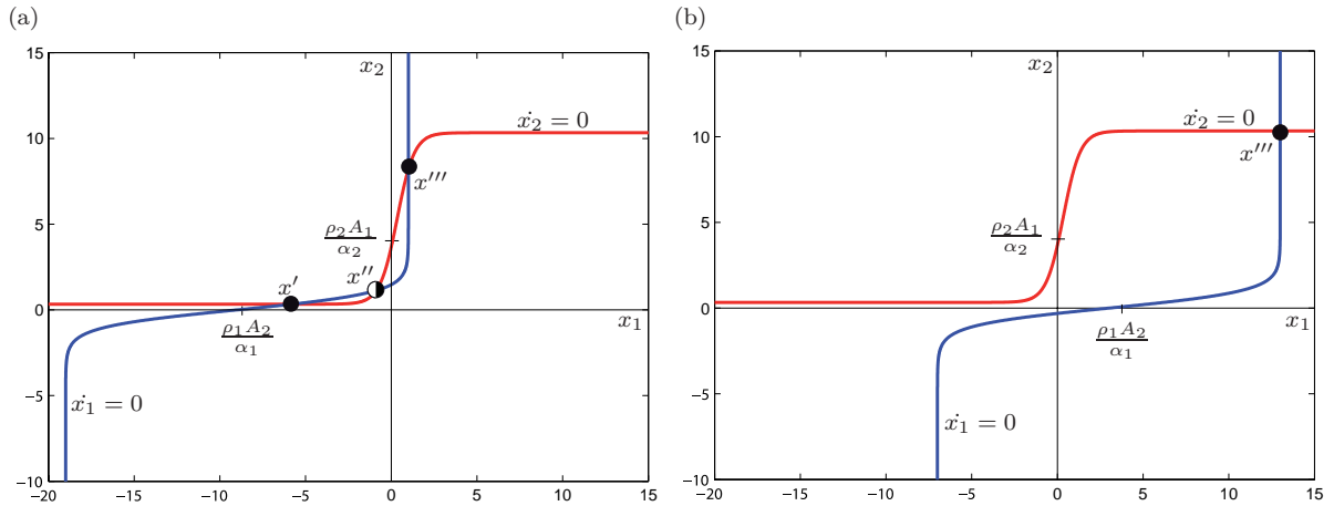
Figure 2: The null-clines \dot{x}_1 = 0 (blue) and \dot{x}_2 = 0 (red) for R_1 and R_2 as in Figure 1, \rho_1 = 0.5 , \rho_2 = 1 , \alpha_1 = 0.1 , \alpha_2 = 0.3 , A_1 = 1.05 , and (a) A_2 = -1.9 : three equilibria x' , x'' , and x''' ; (b) A_2 = 0.5 : one equilibrium x''' .
