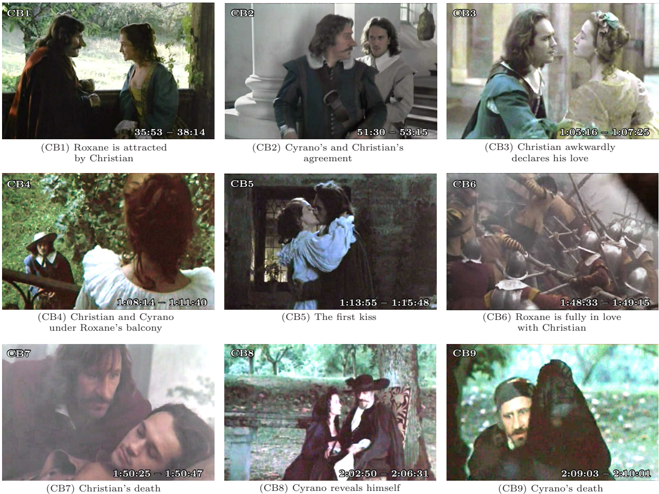
Figure 6: Still frames of the nine film segments (CB1,...,CB9) described in the text. Source: home.dei.polimi.it/rinaldi/CyranoDeBergerac/film.html , where the corresponding original text of the play (in French) and its translation in English can also be found.
