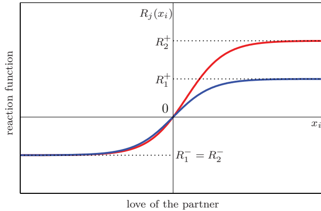
Figure 1: Typical reaction functions R_1(x_2) (blue) and R_2(x_1) (red) of two secure individuals (see Rinaldi et al. [2010]). The two graphs correspond to R_1(x_2) = \frac{e^{x_2} - e^{-x_2}}{e^{x_2}/R_1^+ - e^{-x_2}/R_1^-} and R_2(x_1) = \frac{e^{x_1} - e^{-x_1}}{e^{x_1}/R_2^+ - e^{-x_1}/R_2^-} ; with R_1^+ = 1 , R_2^+ = 2 , and R_1^- = R_2^- = -1 . These two functions are used in the following to describe Roxane and Cyrano.
