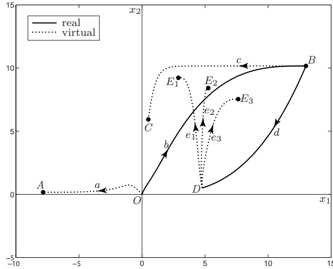
Figure 7: Trajectories of the feelings in each phase (a), . . . , (e) described in the text: (a) virtual no bluffing phase; (b) bluffing phase; (c) virtual phase of no bluffing after Christian's death; (d) separation phase; (e) virtual phase of no bluffing after Roxane's discovery of the truth in the convent: the three trajectories e_1 , e_2 , and e_3 are obtained with sensitivities \rho_1 and \rho_2 reduced of 25%, 50%, and 75%.
