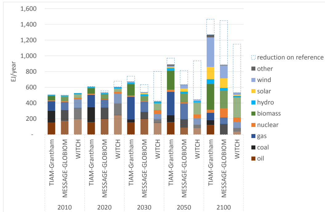
Figure 6: Global primary energy demand to 2100 (2°C scenario, global mitigation action delayed until 2020)
