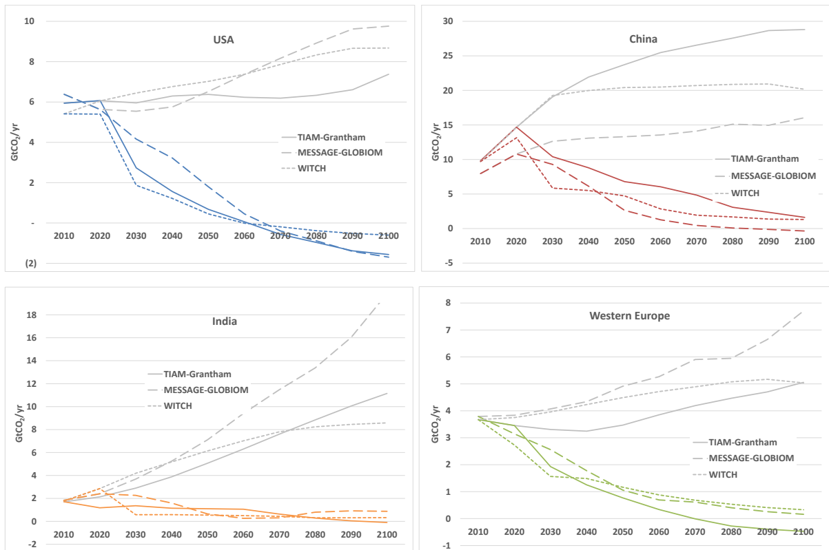
Figure 4: Global CO 2 emissions in reference and 2°C scenario with global mitigation action delayed until 2020, for four major world regions
