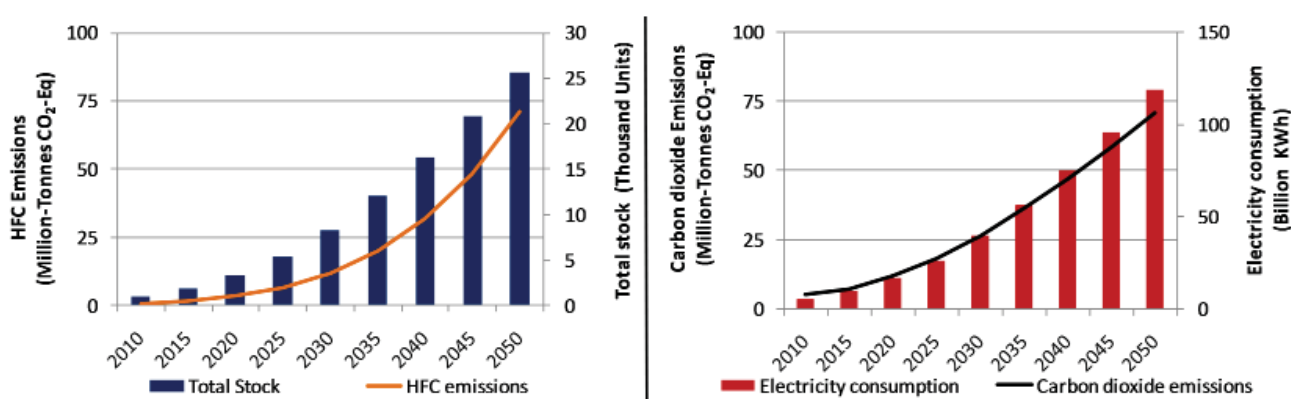
Figure 9: Commercial refrigeration-stocks, electricity consumption and emissions
