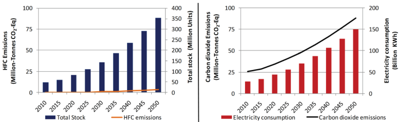
Figure 6: Residential refrigerator-stocks, electricity consumption and emissions
