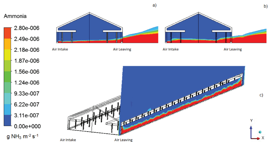
Figure 7. Typical distribution of ammonia flux inside and outside of the opening poultry house: (a) effect with pillars; (b) effect without pillars at the center of the building; (c) plane at the lateral wall.
