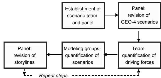
Figure 1. The interaction between the qualitative and quantitative scenario development in the SAS (story and simulation) approach (simplified from Alcamo, 2008).
