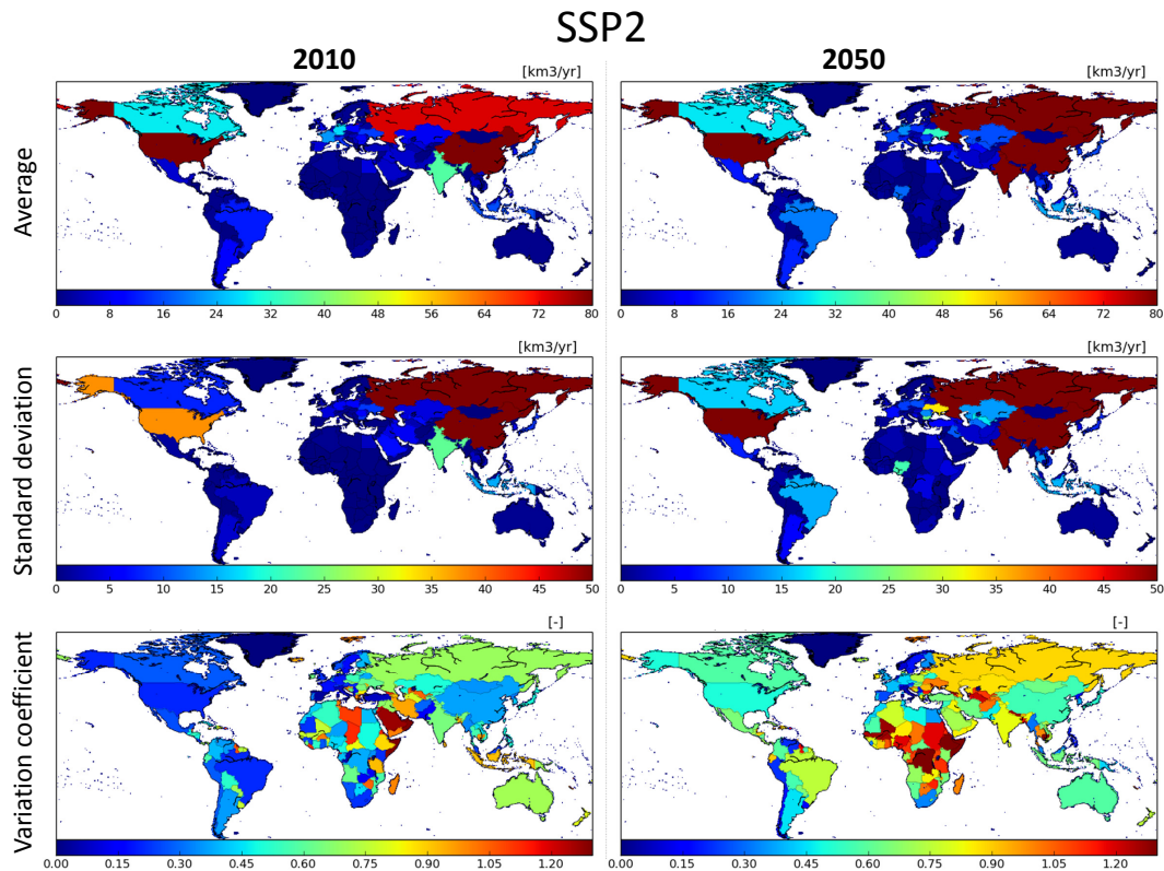
Figure 7. Global maps of projected industrial water withdrawals calculated by the global water models H08, PCR-GLOBWB, and WaterGAP for the years 2010 and 2050, respectively, under the SSP2 scenario. Avr, Std, and Std/Avr denote average, standard deviation, and coefficient of variations.
