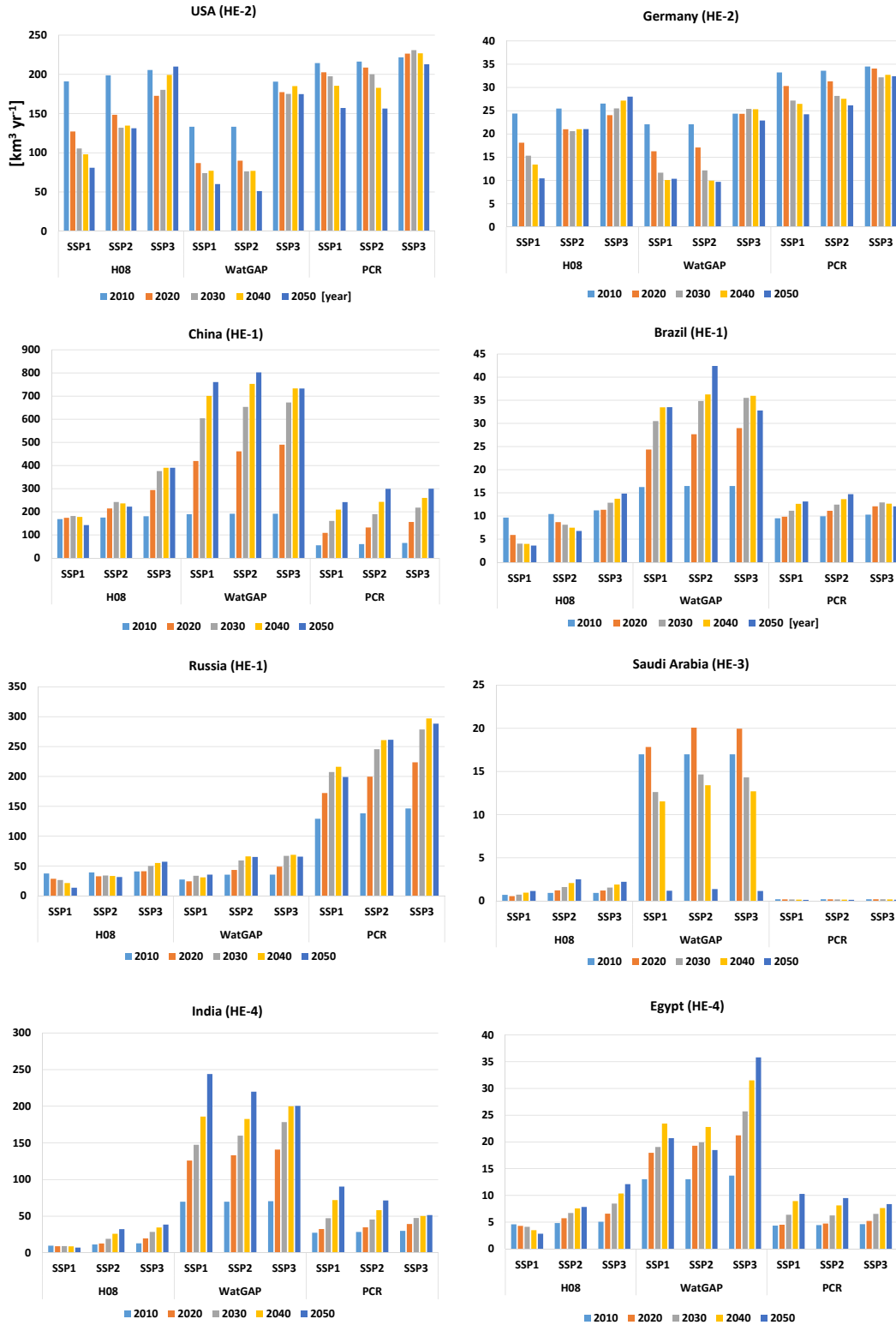
Figure 3. Industrial water withdrawal projections for selected countries calculated by the global water models H08, WaterGAP (WatGAP), and PCR-GLOBWB (PCR) for the years 2010, 2020, 2030, 2040, and 2050, respectively, under three SSP scenarios (SSP1, SSP2, and SSP3). HE denotes the hydro-economic classification (see Appendix A2).
