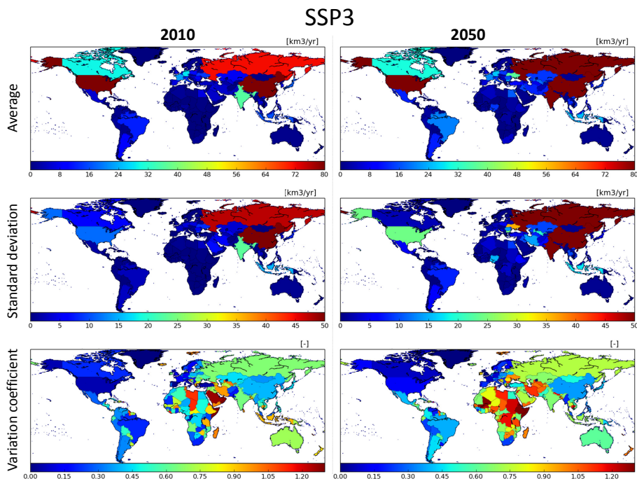
Figure A6. Global maps of projected industrial water withdrawals calculated by the global water models H08, PCR-GLOBWB, and WaterGAP for the years 2010 and 2050, respectively, under the SSP3 scenario. Avr, Std, and Std/Avr denote average, standard deviation, and coefficient of variations.
