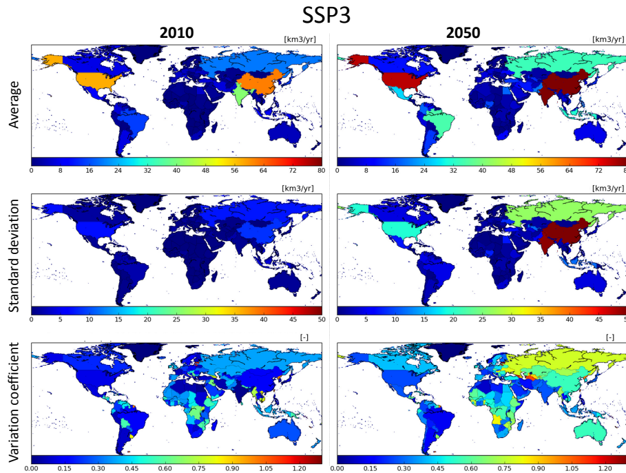
Figure A4. Global maps of projected domestic water withdrawals calculated by the global water models H08, PCR-GLOBWB, and WaterGAP for the years 2010 and 2050, respectively, under the SSP3 scenario. Avr, Std, and Std/Avr denote average, standard deviation, and coefficient of variations (CV).
