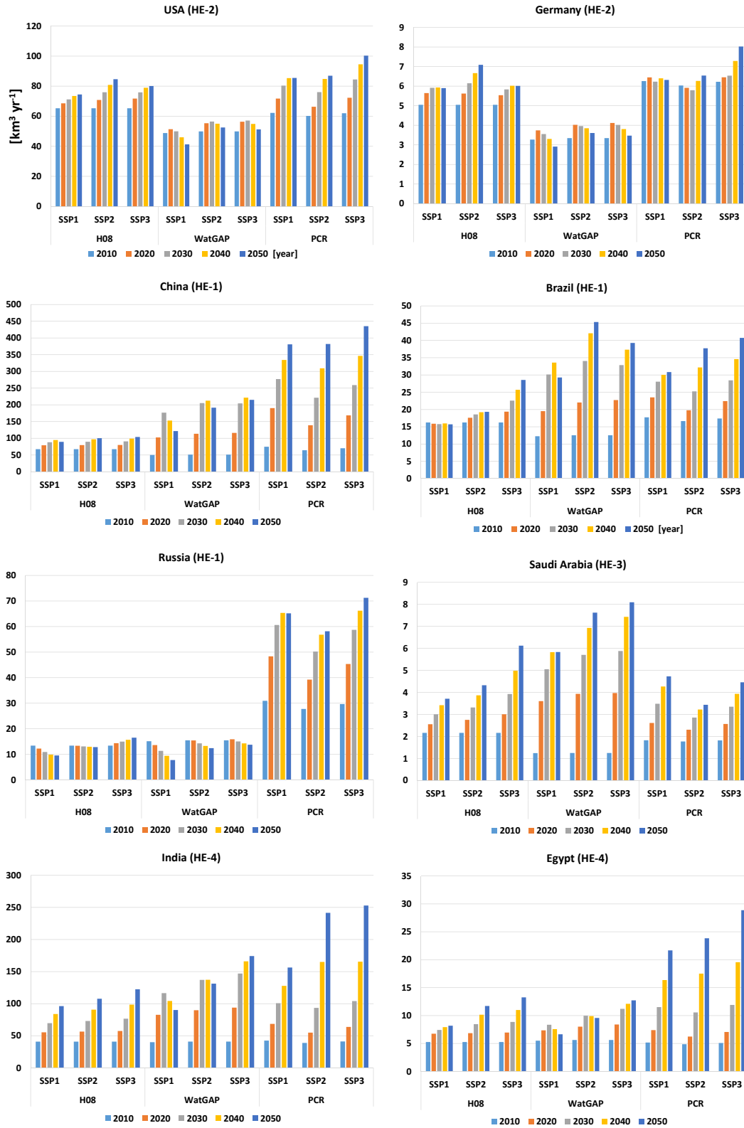
Figure 5. Domestic water withdrawal projections for selected countries calculated by the global water models H08, WaterGAP (WatGAP), and PCR-GLOBWB (PCR) for the years 2010, 2020, 2030, 2040, and 2050, respectively, under three SSP scenarios (SSP1, SSP2, and SSP3). HE denotes the hydro-economic classification (see Appendix A2).
