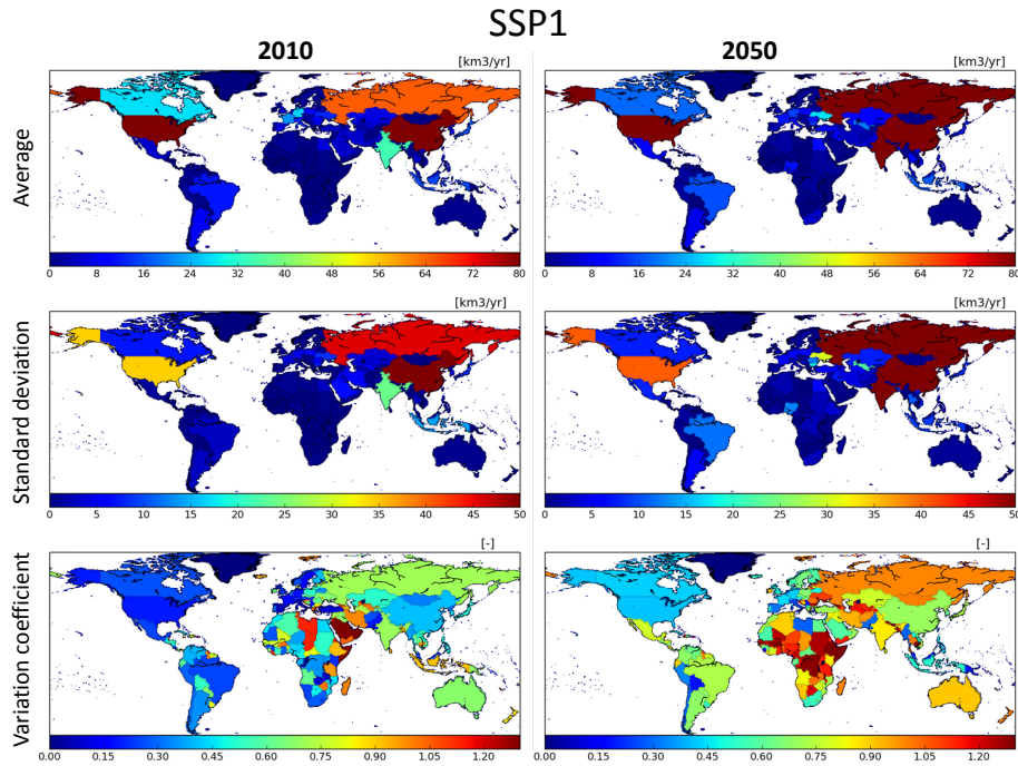
Figure A5. Global maps of projected industrial water withdrawals calculated by the global water models H08, PCR-GLOBWB, and WaterGAP for the years 2010 and 2050, respectively, under the SSP1 scenario. Avr, Std, and Std/Avr denote average, standard deviation, and coefficient of variations.
