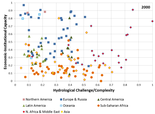
Figure A1. Hydro-economic (HE) classification of countries according to their level of hydrological complexity ( x axis) and their economic-institutional coping capacity ( y axis).
