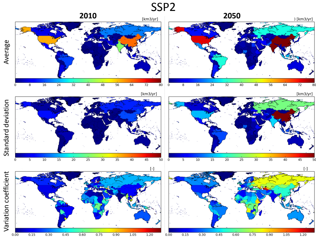
Figure 6. Global maps of projected domestic water withdrawals calculated by the global water models H08, PCR-GLOBWB, and WaterGAP for the years 2010 and 2050, respectively, under the SSP2 scenario. Avr, Std, and Std/Avr denote average, standard deviation, and coefficient of variations (CV).
