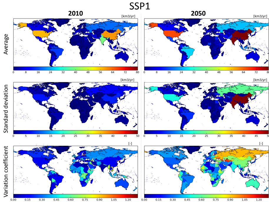
Figure A3. Global maps of projected domestic water withdrawals calculated by the global water models H08, PCR-GLOBWB, and WaterGAP for the years 2010 and 2050, respectively, under the SSP1 scenario. Avr, Std, and Std/Avr denote average, standard deviation, and coefficient of variations (CV).
