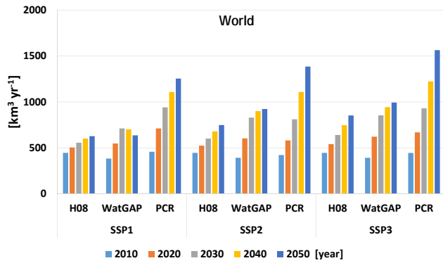
Figure 4. Global domestic water withdrawal projections calculated by the global water models H08, WaterGAP (WatGAP), and PCR-GLOBWB (PCR) for the years 2010, 2020, 2030, 2040, and 2050, respectively, under three SSP scenarios (SSP1, SSP2, and SSP3).
