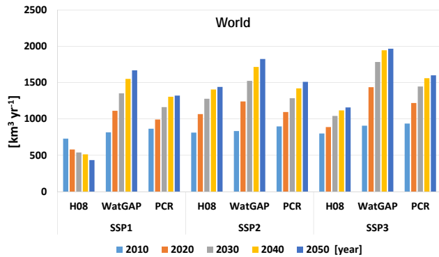
Figure 2. Ensemble of three global industrial water withdrawal projections calculated by the global water models H08, WaterGAP (WatGAP), and PCR-GLOBWB (PCR) for the years 2010, 2020, 2030, 2040, and 2050, respectively, under three SSP scenarios (SSP1, SSP2, and SSP3).
