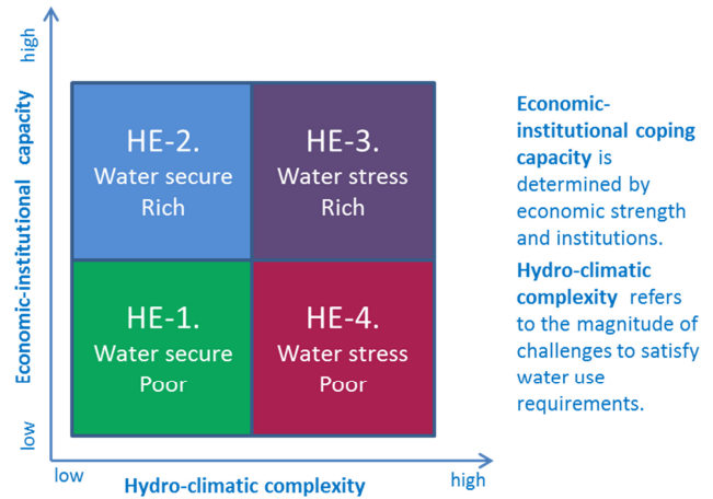
Figure A2. Hydro-economic (HE) quadrants for human–natural water development challenges.
