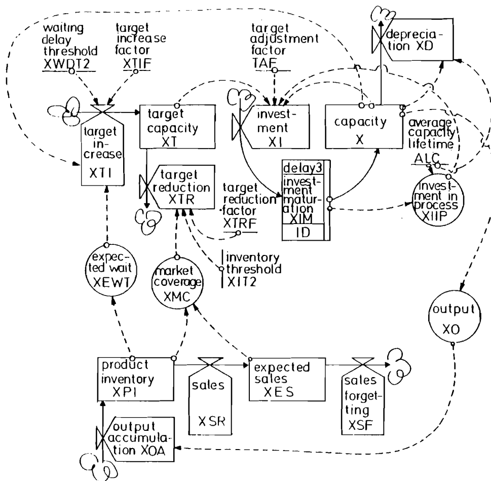
Figure 3: Investment structure used in PLANMKT
