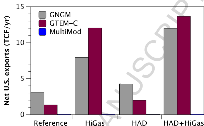
Figure 7. U.S. natural gas export levels in 2040 across three models for all scenarios.
