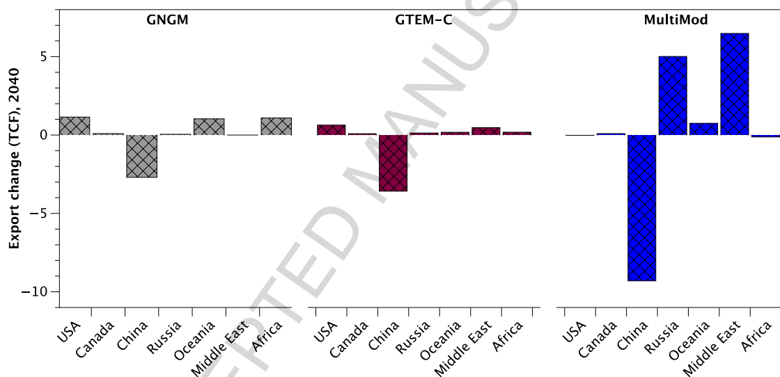
Figure 6. Export change in HAD scenario compared with the Ref scenario in 2040.
