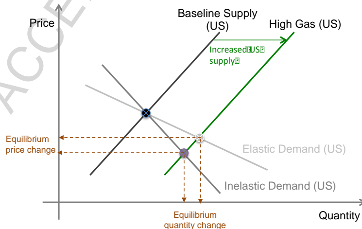
Figure 1. Shifts in the U.S. supply curve in the HiGas scenario.
