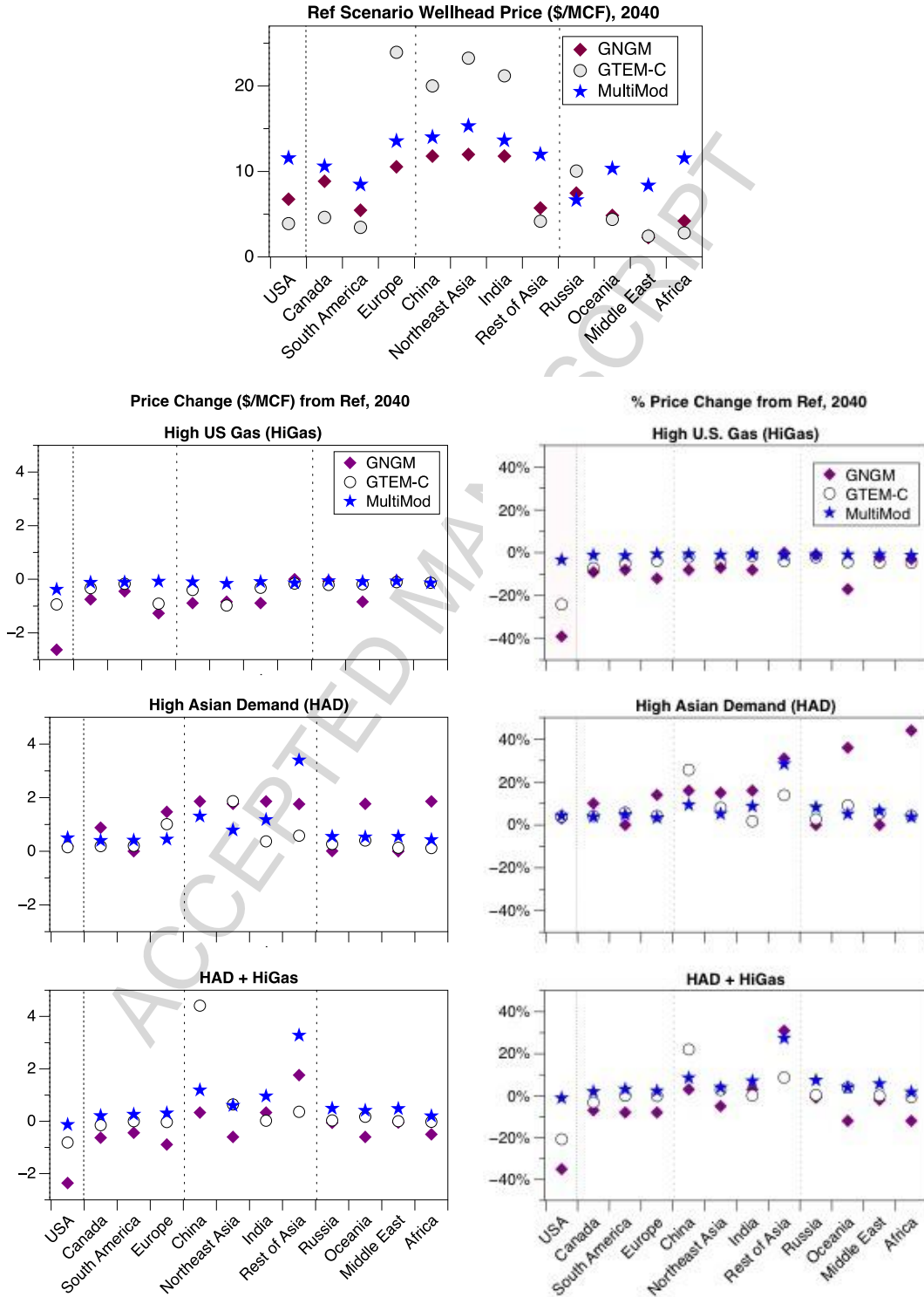
Figure 3. Natural gas wellhead price (top) and price changes in alternative scenarios compared with the Ref scenario in 2040. Left: absolute change. Right: percent change.
