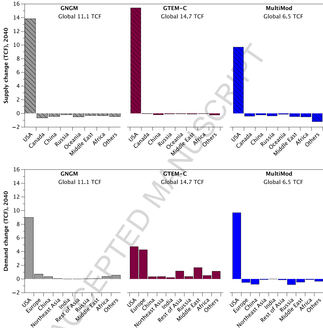
Figure 2. Production (top) and demand changes (bottom) in HiGas scenario compared with the Ref scenario in 2040. Numbers shown below the model names are the total changes globally.
