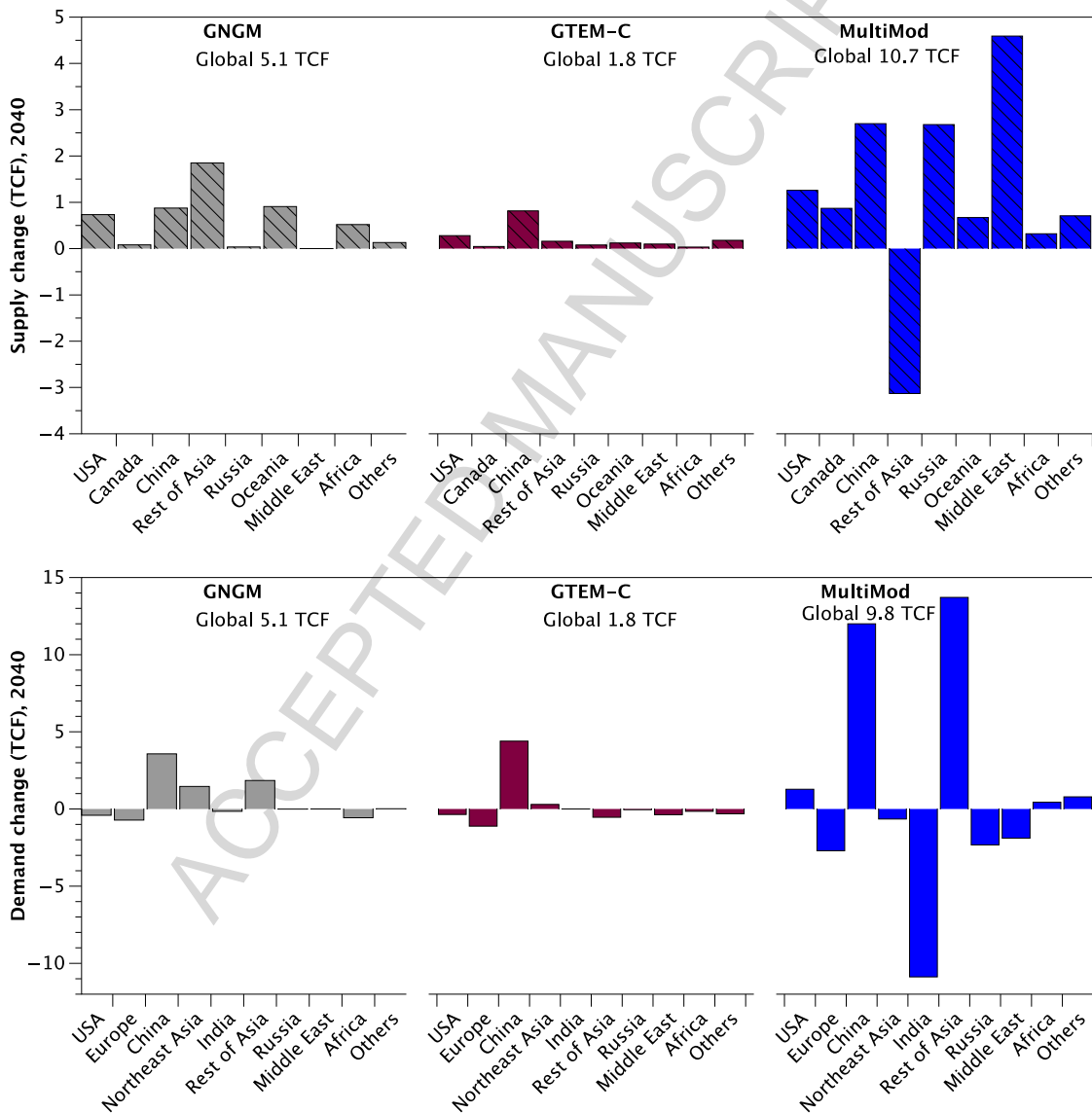
Figure 5. Demand change in HAD scenario compared with the Ref scenario in 2040. Numbers below model names are the net total demand changes globally.
