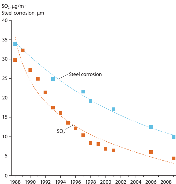
Figure 16. Trends in average corrosion rates and SO 2 concentration between 1988 and 2008 at 20 ICP monitoring sites in Europe (Tidblad et al., 2014).
