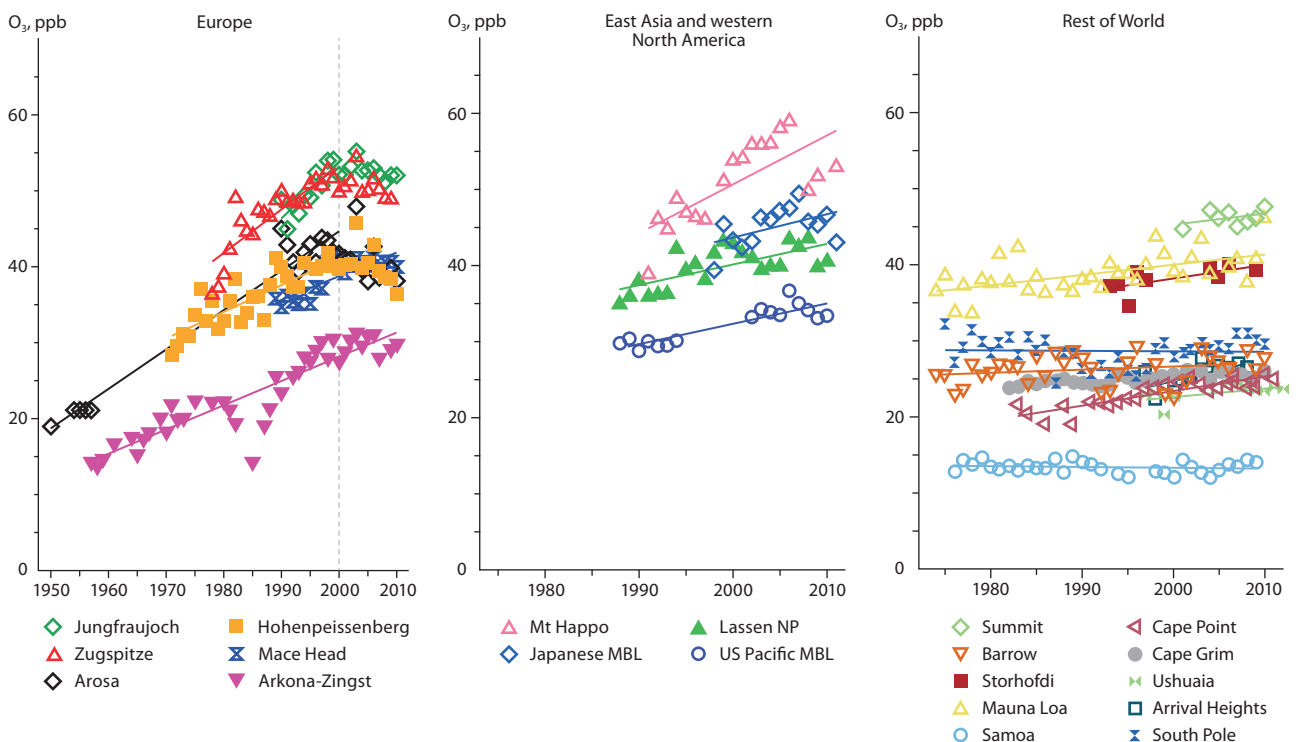
Figure 23. Surface ozone (O 3 ) time series at several rural sites around the world. Trend lines are fitted through the annual average O 3 values using the linear least-square regression method. Trend lines in Europe extend only through 2000 at which point the positive trend appears to end (Cooper et al. 2014).
