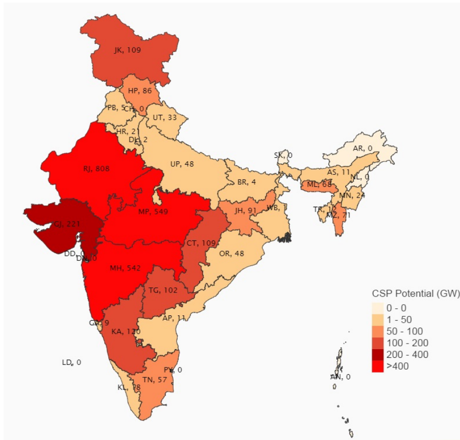
a) CSP potential at an WPD ≥ 150 W/m 2
