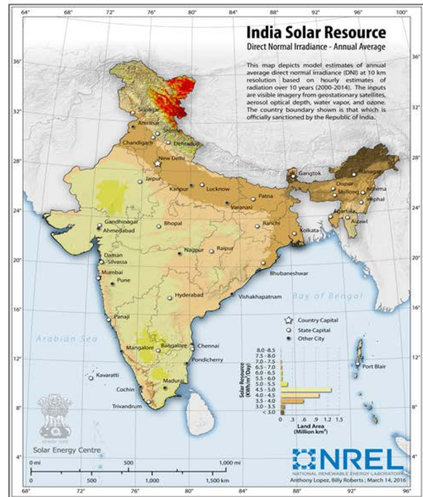
(b) Direct normal solar irradiance
