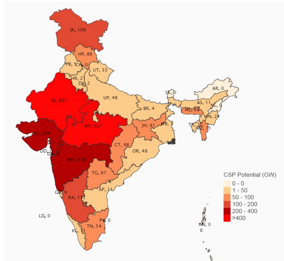
b) CSP potential at an WPD ≥ 200 W/m 2
