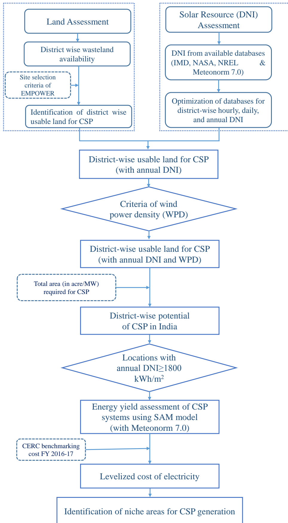
Fig. 6: Methodology adopted for district-wise CSP potential assessment and identification of niche areas for CSP systems in India.
