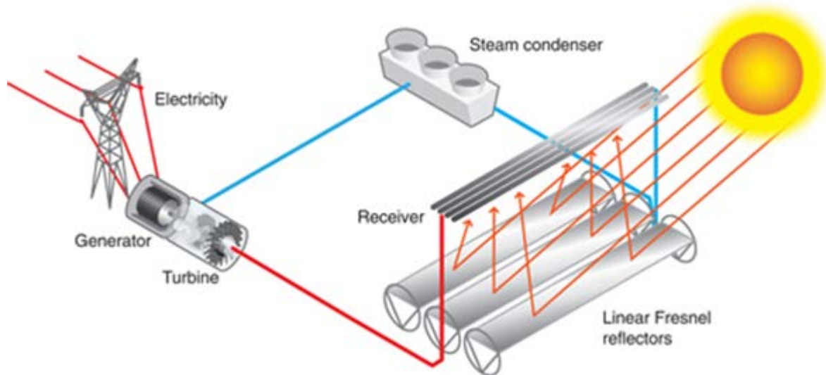
Fig. 3: A linear Fresnel reflector power plant
