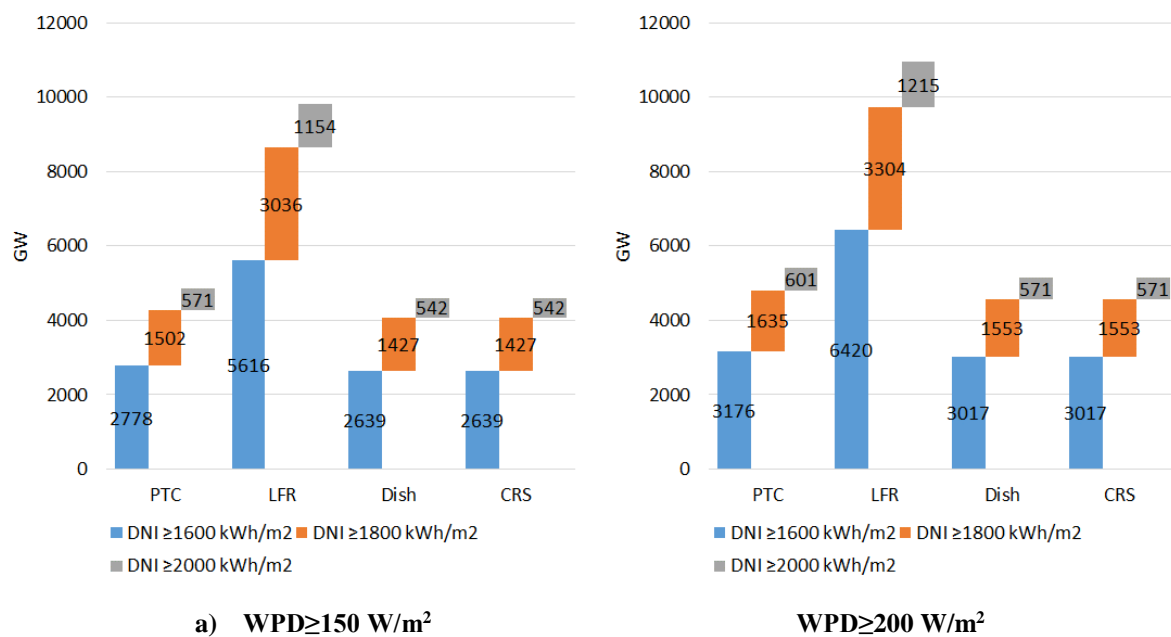
Fig. 9: CSP potential in India at with different DNI and WPD criterion
