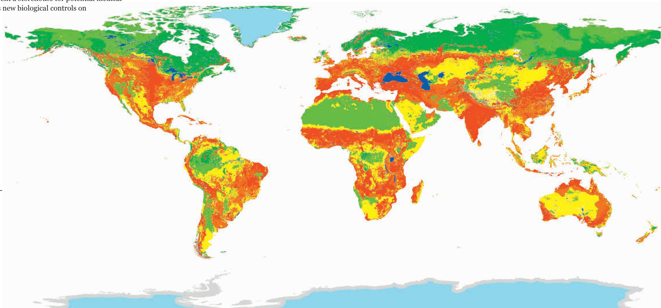
Figure 9: Global map showing the distribution of potential threats to soil biodiversity
