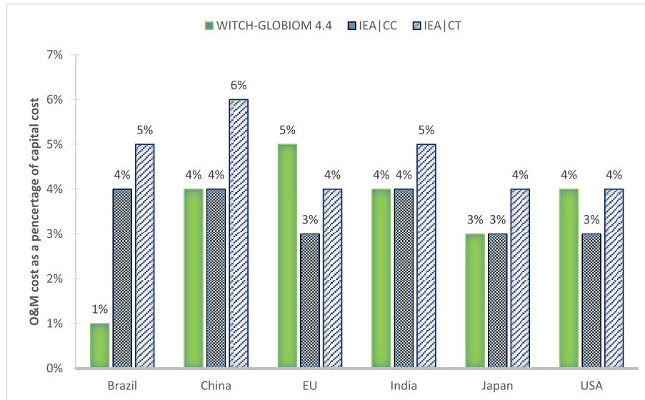
Fig. 7. O&M cost as a percentage of capital cost for gas power plants – varying across regions.
