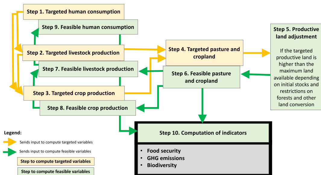
Figure 4 Overview of the FABLE Calculator
