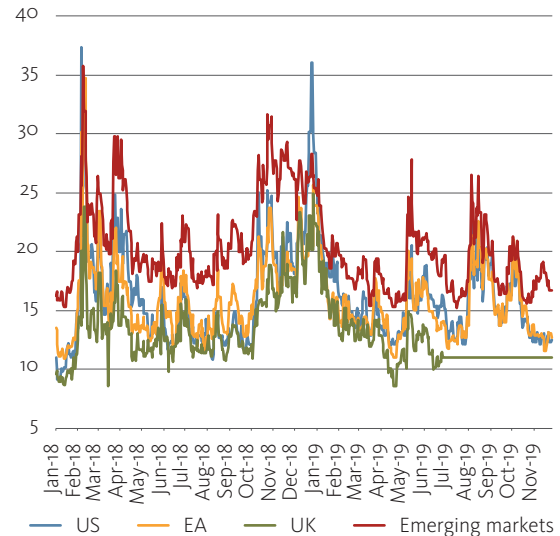
Figure 1.12: Market volatilities
