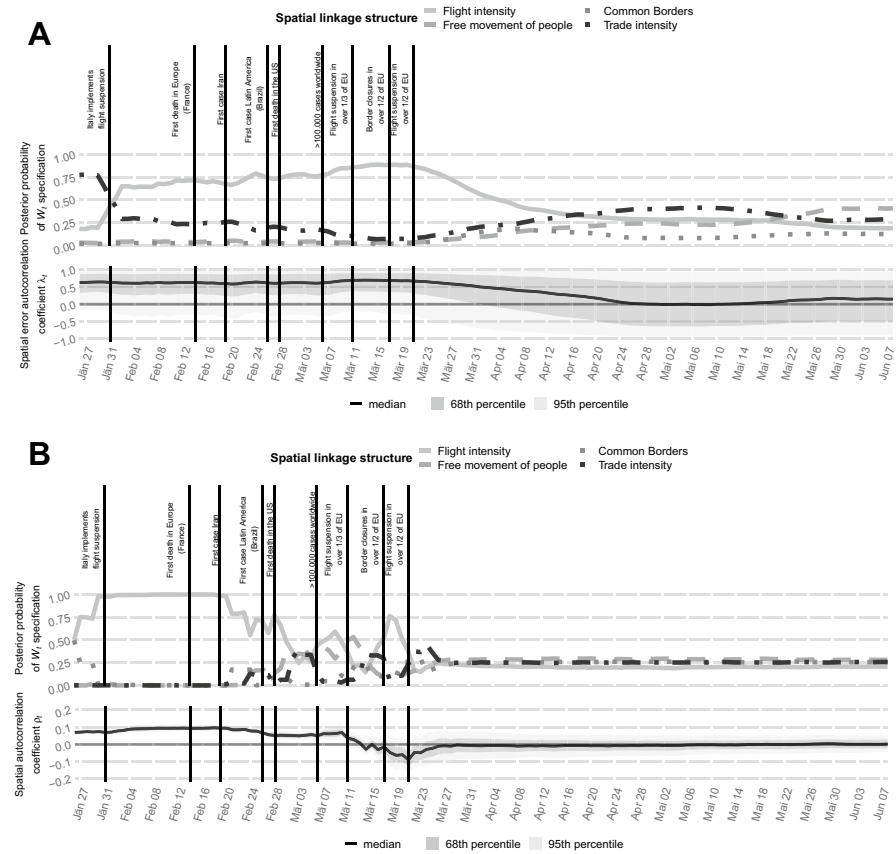
Fig. 2 Posterior parameter estimates for the spatial dynamic panel SAR (i) and Poisson SEM (ii) specifications. Top panels indicate posterior inclusion probability of spatial weight matrices over time. Bottom panels indicate the smoothed posterior median of the spatial autoregressive parameter \rho_i and \lambda_i , respectively
