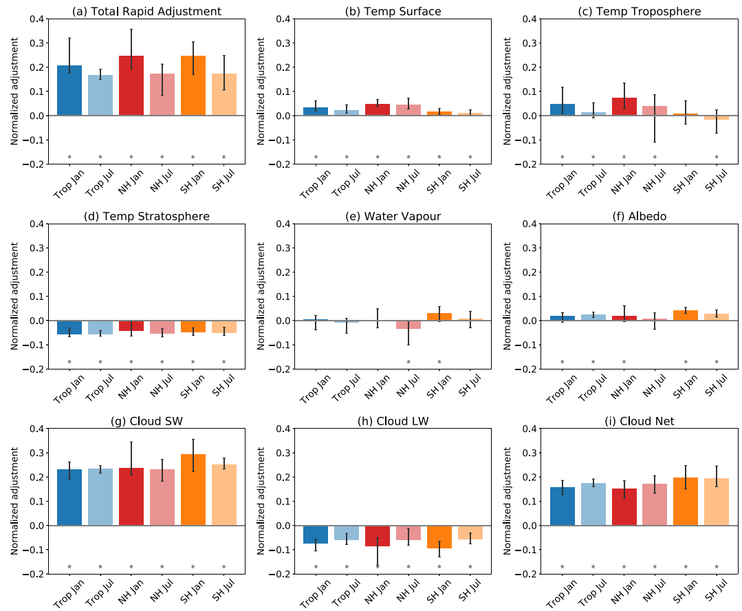
Figure 3. Time-integrated global mean rapid adjustments (a–i) averaged across the different eruption subsets. Rapid adjustments in each simulation were divided by the magnitude of the time-integrated global mean IRF (keeping positive rapid adjustments positive). The total rapid adjustment is shown in Figure 3a, and the remaining subplots show the breakdown of the total rapid adjustment into the contributing components. Error bars show the range in the rapid adjustments among the eruptions in each subset. Stars indicate where the adjustment is significant at the 95% confidence level according to a two-sided Student’s t test.
