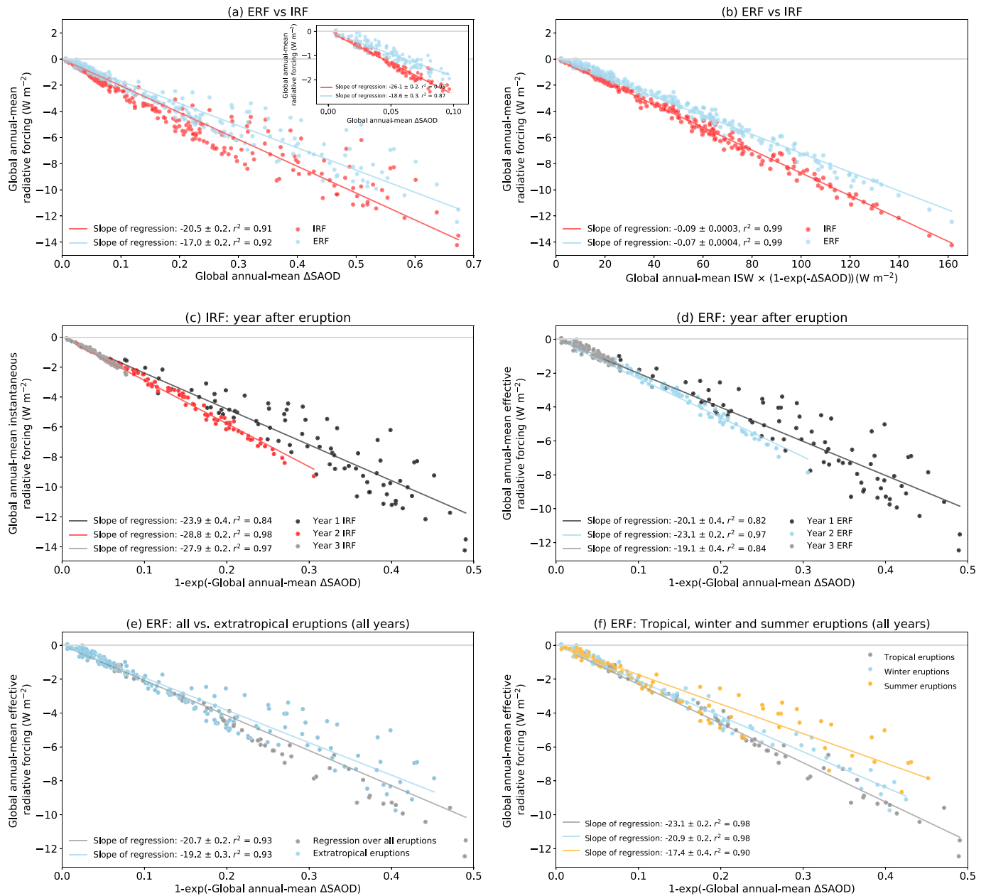
Figure 1. (a) Regression of global annual-mean volcanic SAOD (at 550 nm) against the IRF (red) and ERF (blue) for all 82 simulations. The scatter points show the two quantities in each of the 3 years after each eruption (82 simulations × 3 years giving 246 data points). The inset shows the regression for SAOD values less than 0.1, upon which the IPCC AR5 scaling factor is based. (b) Global annual mean of 1 - e^{-\text{SAOD}} multiplied by the incoming shortwave radiation (ISW), against IRF and ERF. (c) 1 - e^{-\text{SAOD}} against IRF for each year after the eruption. (d) As (c), but for ERF. (e) As (d), but for all and extratropical eruptions for all years. (f) As (d), but for tropical, winter, and summer eruptions for all years. The IRF is shown in Figure S1.
