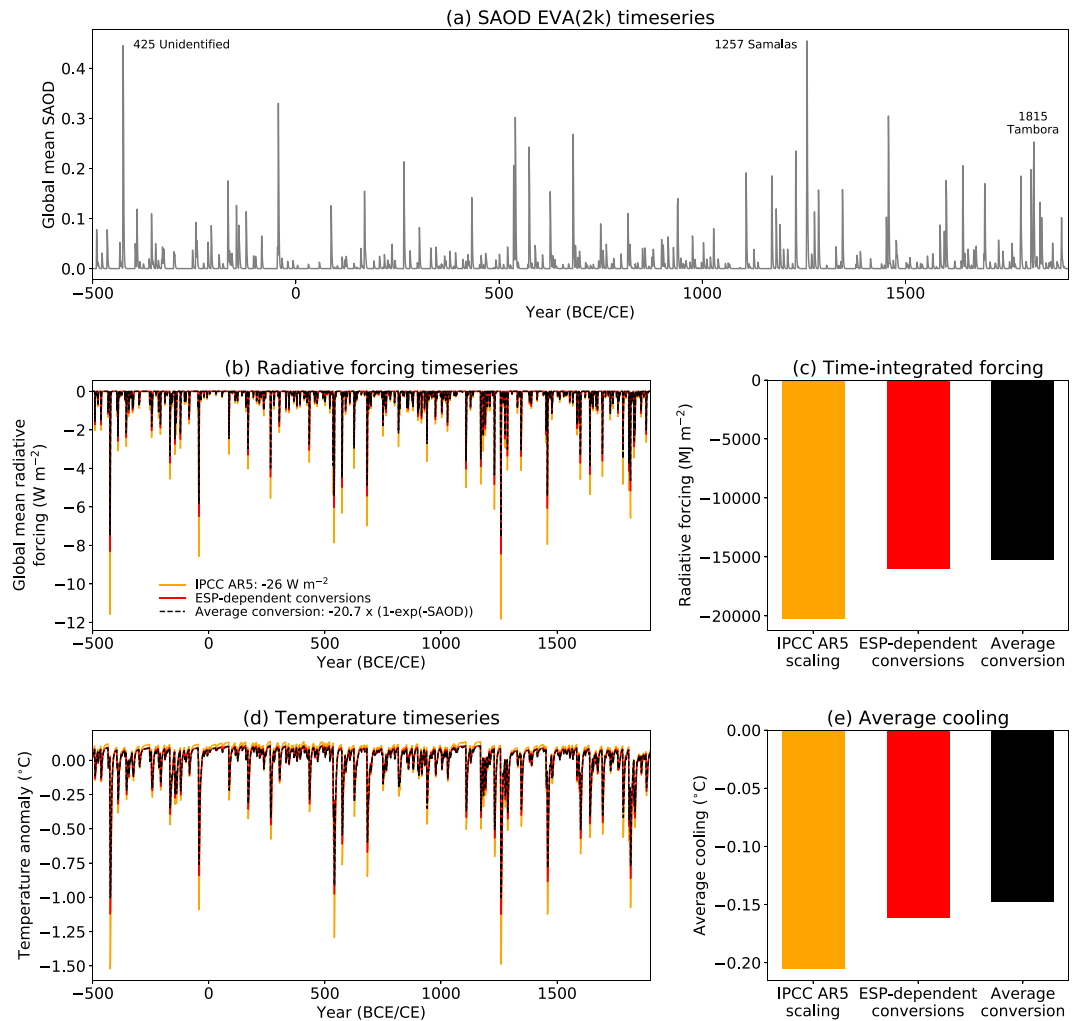
Figure 2. (a) Global annual-mean volcanic SAOD time series from the EVA(2k) reconstruction (calendar years), which does not include background sulfur emissions so that SAOD represents the change due to volcanic eruptions only. (b) Volcanic forcing calculated from the SAOD using the IPCC AR5 scaling factor (orange), eruption source parameter (ESP)-dependent conversions (Table S1) (red), and the all-eruption average conversion (black). (c) Time-integrated forcing from 500 BCE to 1900 CE for the three conversion methods. (d) Global annual-mean surface temperature anomalies (relative to the 2,400-year average from each time series) calculated in a simple climate model (FaIR) for each volcanic forcing time series. (e) The average cooling for temperature anomalies less than 0 for the three conversion methods.
