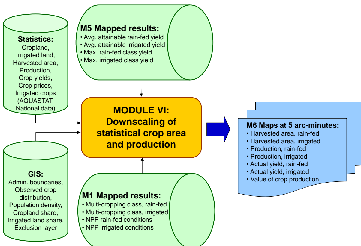
Figure 8-1 Information flow in Module VI
