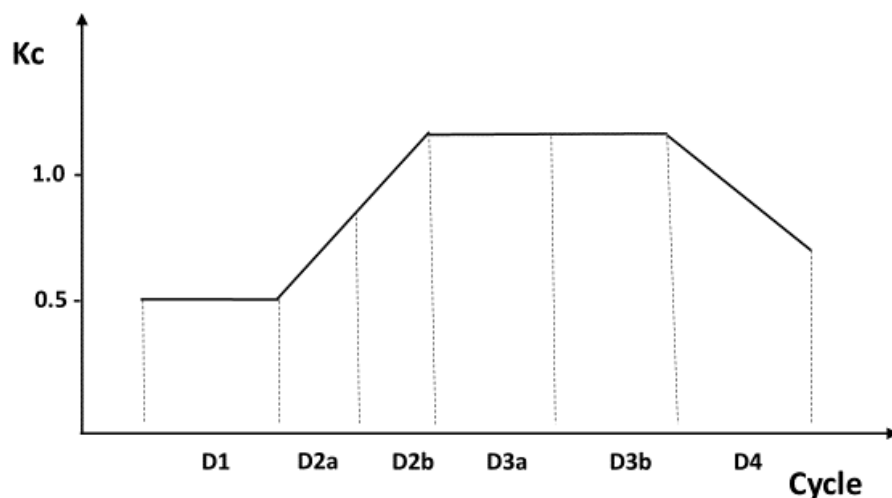
Figure 4-2 Schematic representation of Kc values for different crop development stages
