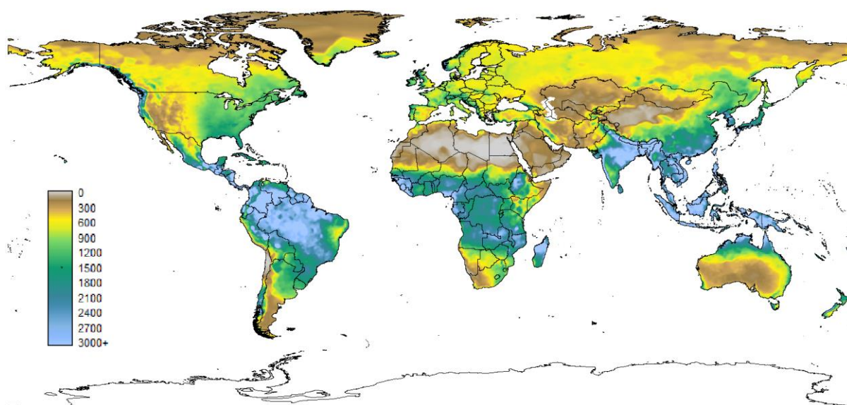
Figure 6-6 Modified Fournier index (Fm)
