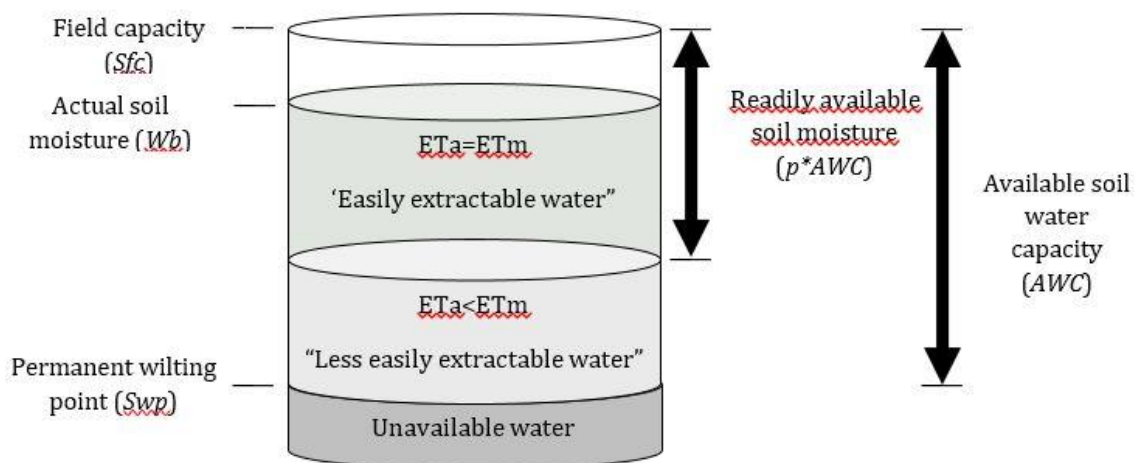
Figure 3-8 Schematic representation of water balance calculations
