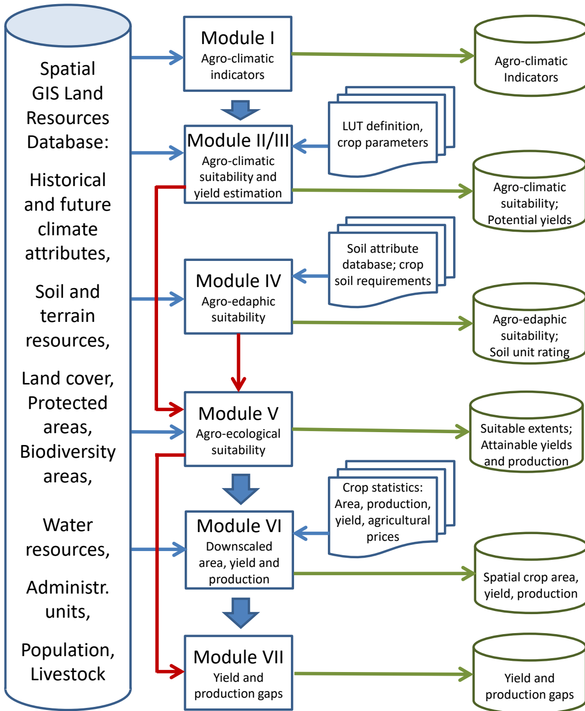
Figure 1-1 Overall structure and data integration of GAEZ v4 (Module I-VII)
