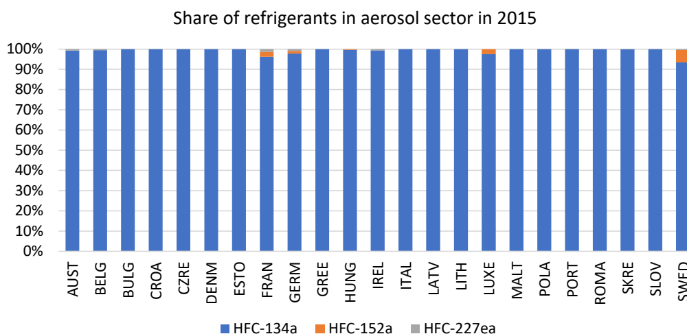
Figure 18: Share of HFC's in aerosol sector of EU countries in 2015
