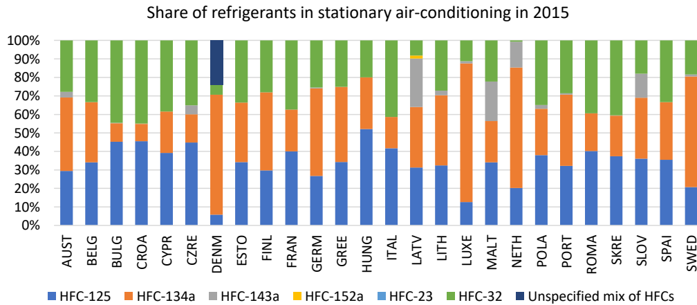
Figure 7: Share of refrigerants in stationary air-conditioning sector in 2015 as reported to UNFCCC (2019).
