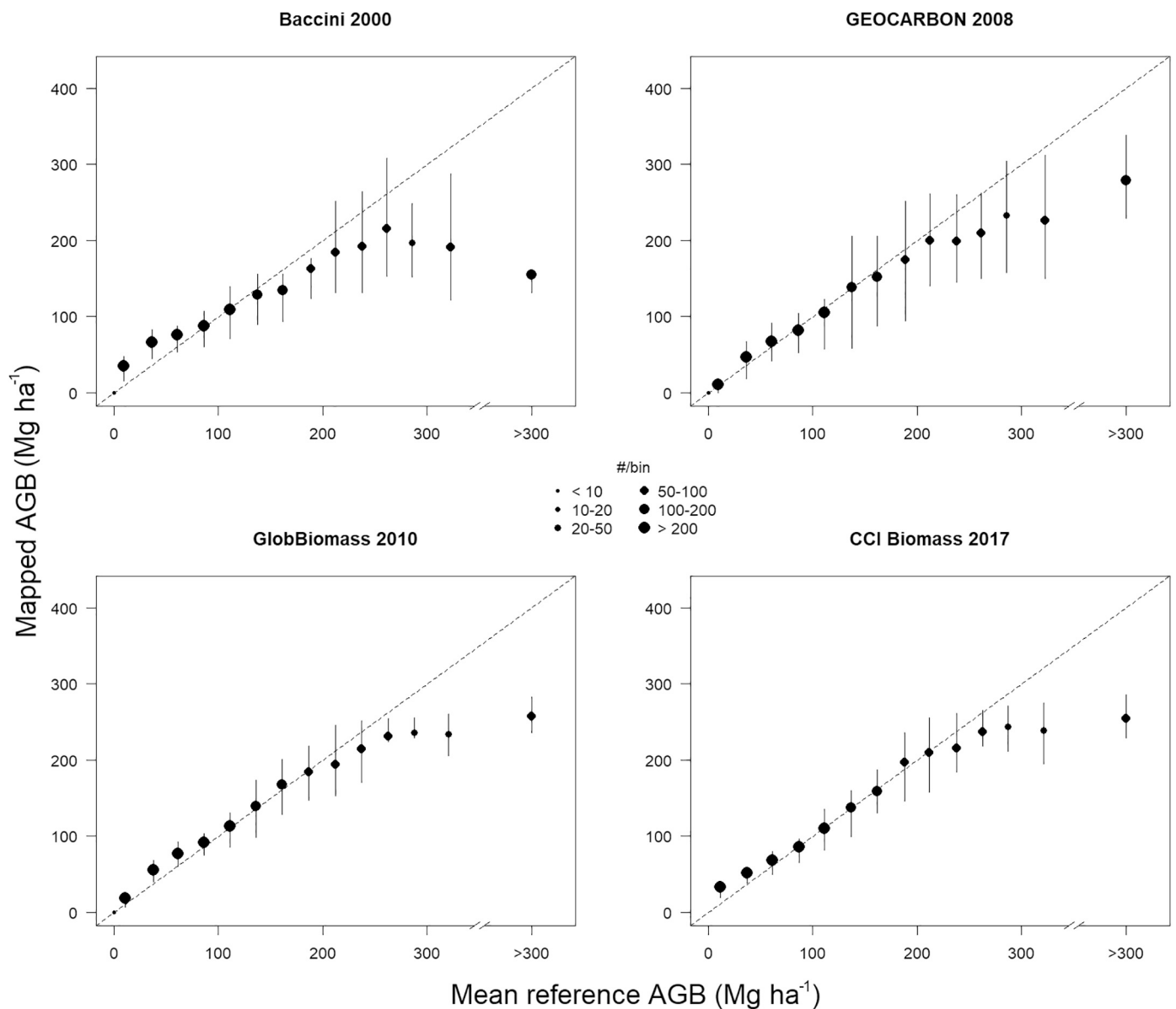
Fig. 4. Map estimates of AGB aggregated to 0.1° against mean plot AGB within 0.1° grid cells for all four AGB maps. The number of grid cells are: Baccini = 6561; GEOCARBON = 6521; GlobBiomass = 6201; and CCI Biomass = 2612 originating from plot datasets \pm 10 years apart than the map epoch (see Section 2.2 and Table S2). Each circle represents an AGB bin and its size denotes the number of grid cells in the bin, while the whiskers correspond to the 25 th and 75 th percentile range of the map AGB.
