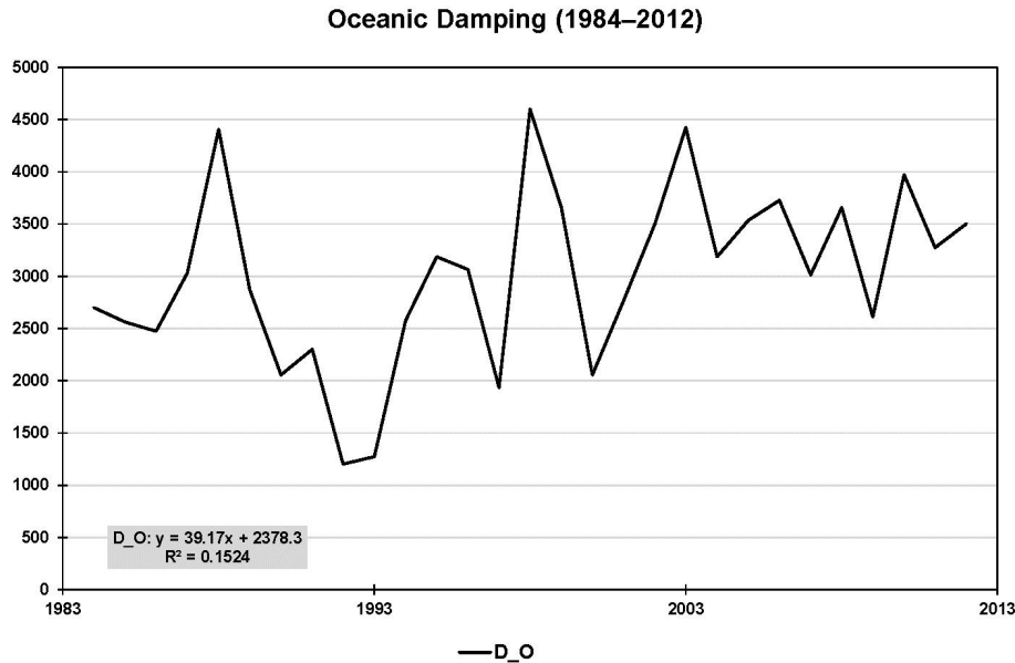
Figure 4. Oceanic carbon uptake perceived as damping (in ppmv yr) based on observations at seven ocean carbon time series sites for periods from 15 to 30 years (between 1983 and 2012). The linear trend in oceanic damping, shown at the bottom, is used to interpret damping as a constant with appropriate uncertainty (given by half the maximal range).
