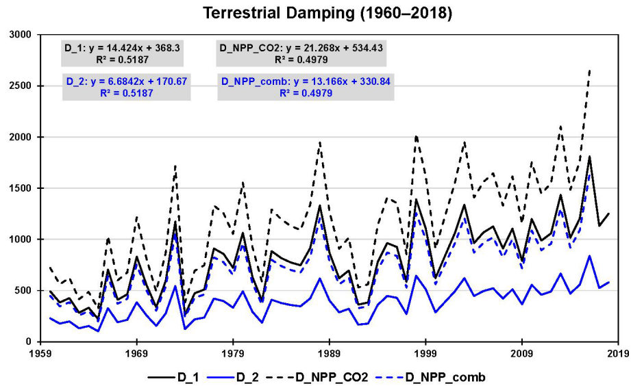
Figure 3. Terrestrial carbon uptake perceived as damping (in ppmv yr) based on the limits of leaf photosynthesis (1960–2018: D_1 and D_2 ) and on model-derived changes in net primary production (NPP; 1960–2016) due to the combined effect of \text{CO}_2 fertilization, nitrogen deposition, climate change, and carbon–nitrogen synergy ( D_{\text{NPP\_comb}} ) as well as \text{CO}_2 fertilization only ( D_{\text{NPP\_CO}_2} ). The linear trends of the four damping series are shown at the top. These are used to interpret damping as constants with appropriate uncertainty (given by half the maximal range).
