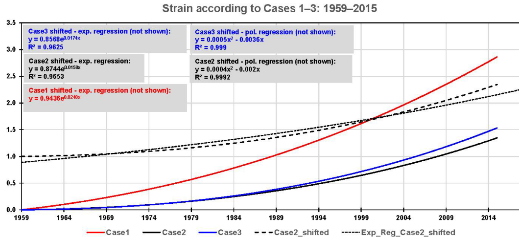
Figure 6. Cases 1–3: the ratio K/D is varied from minimum (Case 1: solid red) to mean (Case 2: solid black) to maximum (Case 3: solid blue) to explore the spread in the strain \varepsilon (in units of 1) on the left side of Eq. (1b), while the monitored stress is described by a second-order polynomial (see the text). These strain responses have to be shifted upward (so that they pass through 1 in 1959) to derive their rates of change if described by an exponential regression (here only demonstrated for Case 2). As is already illustrated in Case 0, the exponential regression in Case 1 is excellent (see the text), whereas second-order polynomial regressions provide better fits in Cases 2 and 3 (see the boxes in the figure; the polynomial regressions are not shown).
