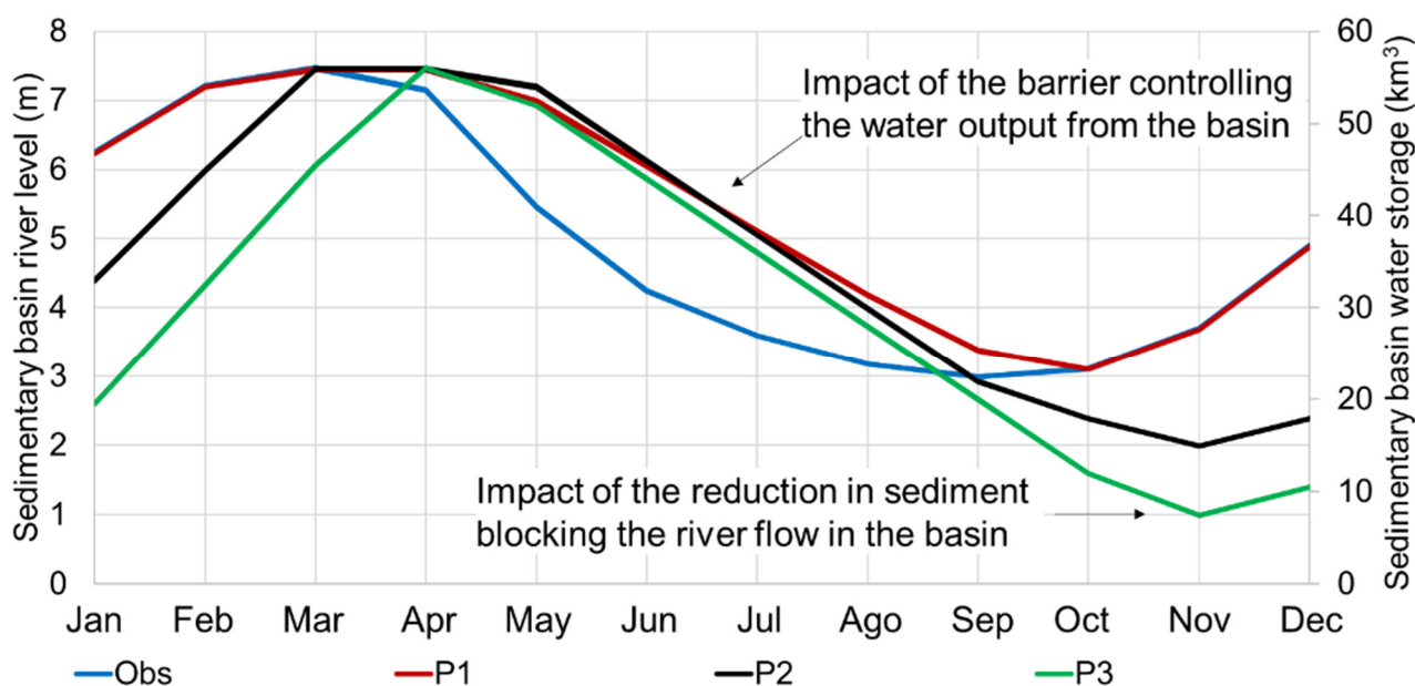
Figure 12. Observed and proposed sedimentary basin river level and water storage.
