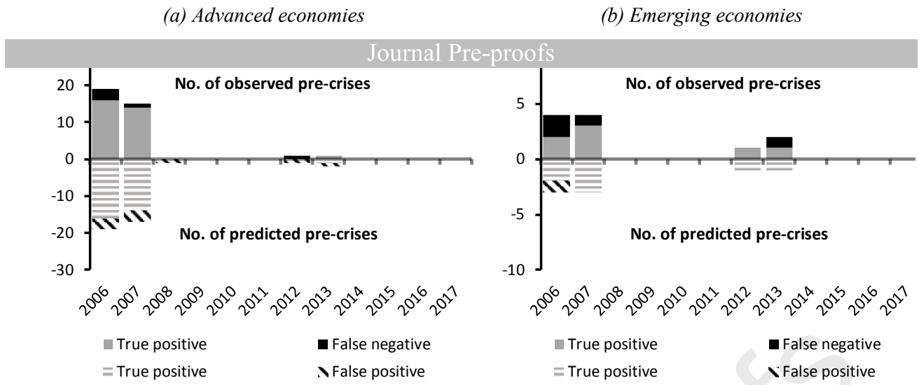
Figure 5 AdaBoost: plot of the confusion matrix by year
