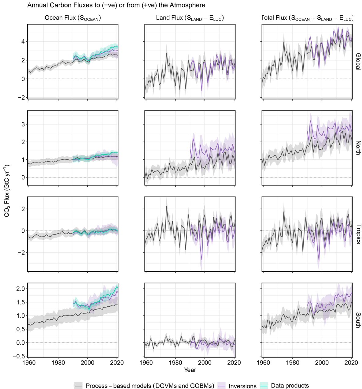
Figure 13. CO 2 fluxes between the atmosphere and the Earth’s surface separated between land and oceans globally and in three latitude bands. The ocean flux is S_{OCEAN} , and the land flux is the net of atmosphere–land fluxes from the DGVMs. The latitude bands are (top row) global, (second row) north ( > 30^\circ N ), (third row) tropics ( 30^\circ S – 30^\circ N ), and (bottom row) south ( < 30^\circ S ), showing values over ocean (left column) and land (middle column) and in total (right column). Estimates are shown for process-based models (DGVMs for land, GOBMs for oceans), inversion systems (land and ocean), and fCO_2 -based data products (ocean only). Positive values indicate a flux from the atmosphere to the land or the ocean. Mean estimates from the combination of the process models for the land and oceans are shown (black line) with \pm 1 standard deviation ( 1\sigma ) of the model ensemble (grey shading). For the total uncertainty in the process-based estimate of the total sink, uncertainties are summed in quadrature. Mean estimates from the atmospheric inversions are shown (purple lines) with their full spread (purple shading). Mean estimates from the fCO_2 -based data products are shown for the ocean domain (light blue lines) with their \pm 1\sigma spread (light blue shading). The global S_{OCEAN} (upper left) and the sum of S_{OCEAN} in all three regions represents the anthropogenic atmosphere-to-ocean flux based on the assumption that the pre-industrial ocean sink was 0 \text{ GtC yr}^{-1} when riverine fluxes are not considered. This assumption does not hold at the regional level, where pre-industrial fluxes can be significantly different from zero. Hence, the regional panels for S_{OCEAN} represent a combination of natural and anthropogenic fluxes. Bias correction and area weighting were only applied to global S_{OCEAN} ; hence, the sum of the regions is slightly different from the global estimate ( < 0.05 \text{ GtC yr}^{-1} ).
