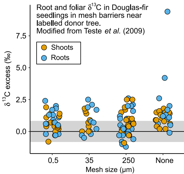
Fig. 4 Data extracted from Teste et al. (2009; figs 2, 3). Root (blue) and foliar (orange) ^{13}\text{C} in Douglas-fir seedlings grown in mesh barriers with various pore sizes, located 0.5 m from labeled donor trees in the field. The x-axis shows the pore size of the mesh barriers, and below it is specified if the barrier is permeable to roots and/or ectomycorrhizal (ECM) fungal hyphae. The 35- \mu\text{m} mesh is designated as allowing 'limited ECM' connectivity, because the pores permit entry of individual hyphae, but not of rhizomorphs. The 250- \mu\text{m} mesh is completely permeable to all ECM fungal hyphae and rhizomorphs but prevents root ingrowth/outgrowth. No significant differences among shoots of different mesh treatments were detected ( P > 0.5 , analysis of variance). A two-way analysis of variance (with mesh size and tissue type as factors) shows only that root \delta^{13}\text{C} was higher than shoots ( P < 0.0001 ) and that 'no mesh' seedlings were more enriched than the seedlings subjected to various mesh treatments ( P < 0.03 ). No significant difference among mesh sizes was detected ( P > 0.78 ). The hypothesis that common mycorrhizal networks (CMNs) enhance C transfer between plants predicts that the 0.5- \mu\text{m} mesh treatment (and possibly also the 35- \mu\text{m} treatment) should receive significantly less ^{13}\text{C} than the other treatments. This was not shown, and so the hypothesis should be rejected in this case.
