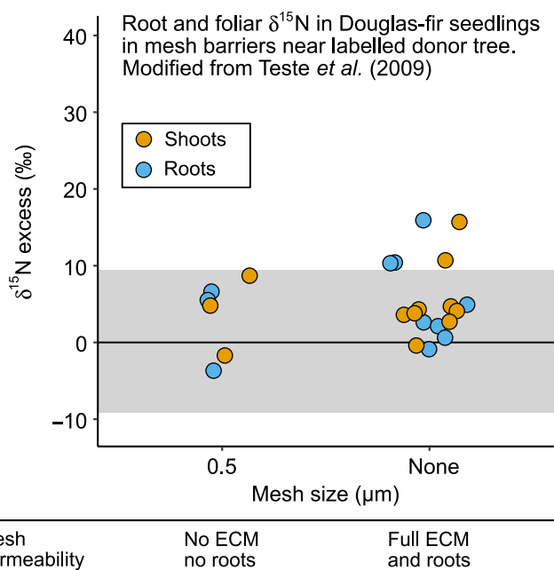
Fig. 5 Data extracted from Teste et al. (2009; fig. 4). Root (blue) and foliar (orange) ^{15}\text{N} in Douglas-fir seedlings in the field, with or without mesh barriers that prevent common mycorrhizal network (CMN) connections to labeled donor trees, 0.5 m away. The x-axis shows the pore size of the mesh barriers, and below it is specified if the barrier is permeable to roots and/or ectomycorrhizal (ECM) fungal hyphae. Student's t -tests performed on the extracted data revealed that the 0.5- \mu\text{m} mesh did not significantly affect seedling ^{15}\text{N} concentration in shoots ( P = 0.65 ) or roots ( P = 0.47 ).
