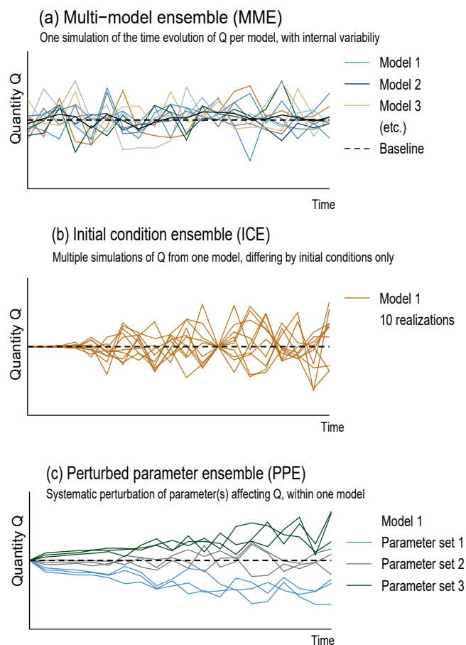
Figure 1.21 | Illustration of common types of model ensemble, simulating the time evolution of a quantity Q (such as global mean surface temperature). (a) Multi-model ensemble, where each model has its own realization of the processes affecting Q, and its own internal variability around the baseline value (dashed line). The multi-model mean (black) is commonly taken as the ensemble average. (b) Initial condition ensemble, where several realizations from a single model are compared. These differ only by minute (‘micro’) perturbations to the initial conditions of the simulation, such that over time, internal variability will progress differently in each ensemble member. (c) Perturbed physics ensemble, which also compares realizations from a single model, but where one or more internal parameters that may affect the simulations of Q are systematically changed to allow for a quantification of the impact of those quantities on the model results. Additionally, each parameter set may be taken as the starting point for an initial condition ensemble. In this figure, each set has three ensemble members.
