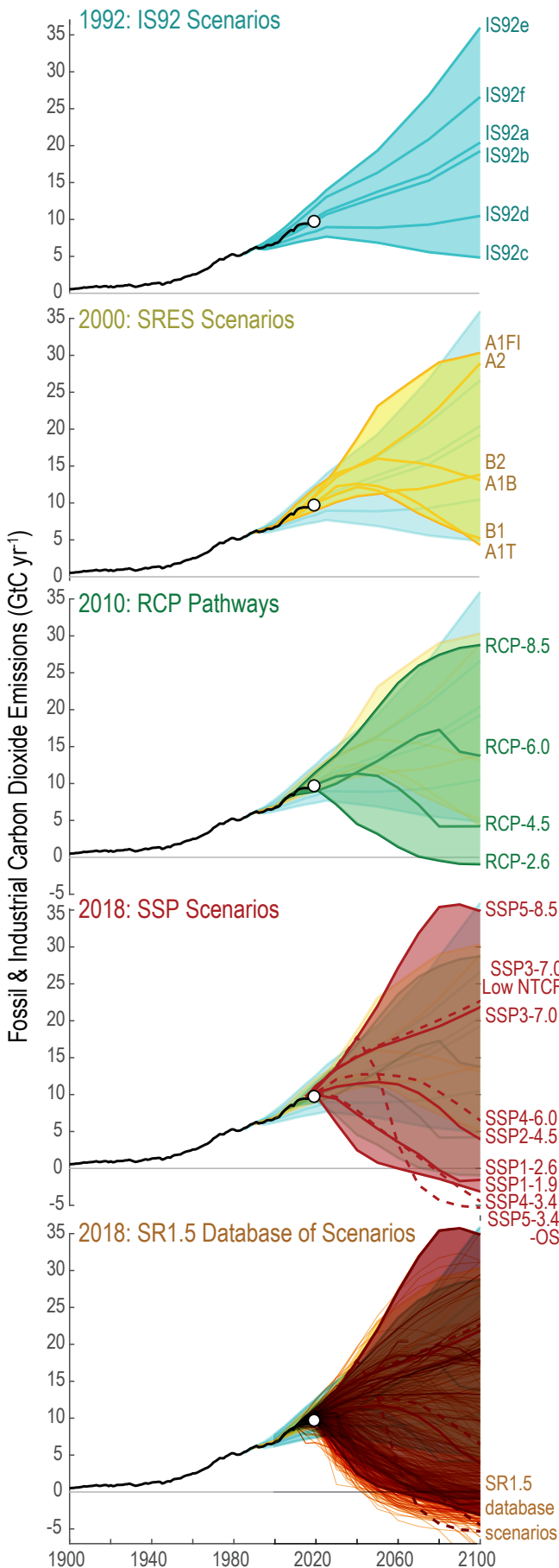
Figure 1.28 | Comparison of the range of fossil fuel and industrial CO 2 emissions from scenarios used in previous assessments up to AR6. Previous assessments are the IS92 scenarios from 1992 ( top ), the Special Report on Emissions Scenarios (SRES) scenarios from the year 2000 ( second panel ), the Representative Concentration Pathway (RCP) scenarios designed around 2010 ( third panel ) and the Shared Socio-economic Pathways (SSP) scenarios ( fourth panel ). In addition, historical emissions are shown (black line; Figure 5.5); a more complete set of scenarios is assessed in SR1.5 ( bottom ); (Huppmann et al., 2018). Further details on data sources and processing are available in the chapter data table (Table 1.SM.1).
