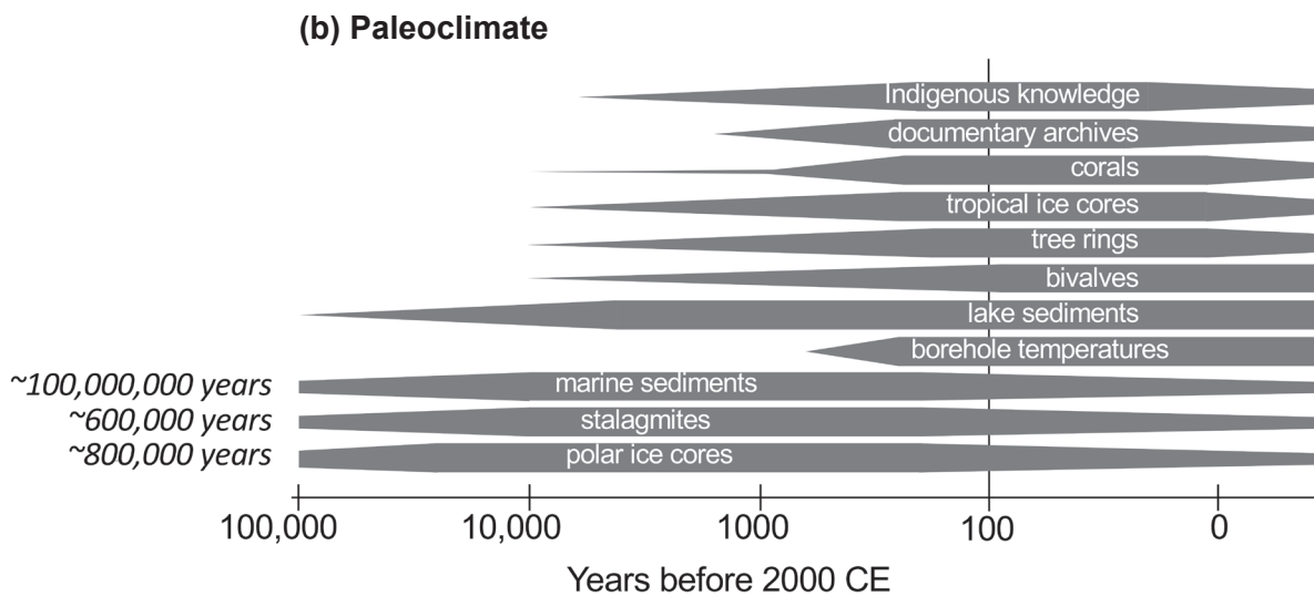
Figure 1.7 | Schematic of temporal coverage of (a) selected instrumental climate observations and (b) selected paleoclimate archives. The satellite era began in 1979 CE. The width of the taper gives an indication of the amount of available records.
