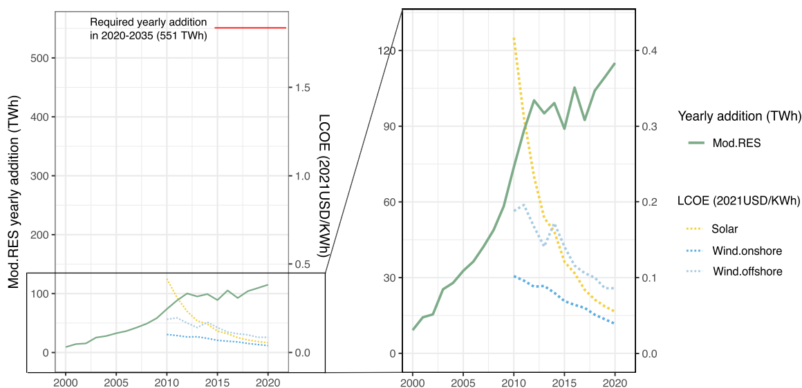
Fig. 4. Costs of solar, onshore, and offshore wind in comparison to yearly addition of modern renewables in the G7 and the EU in 2000–2020 and the required addition in 2020–2035. Note: The costs represent the global weighted average costs of these technologies obtained from IRENA [74].
