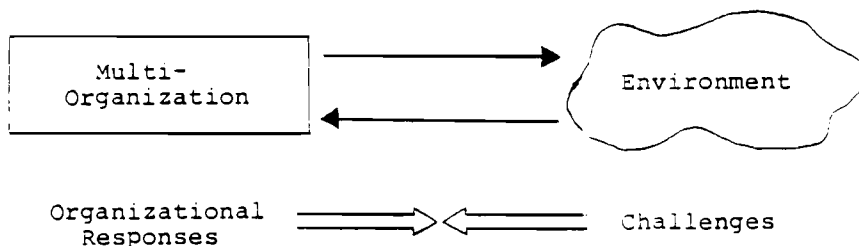
Figure 7. System-environment interaction.
