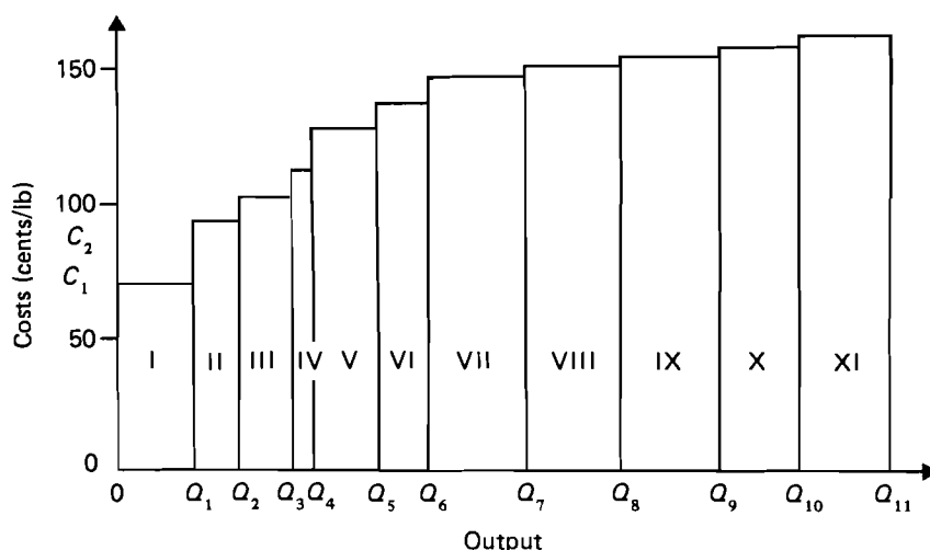
FIGURE 2 Average production costs for existing and potential copper mines.
