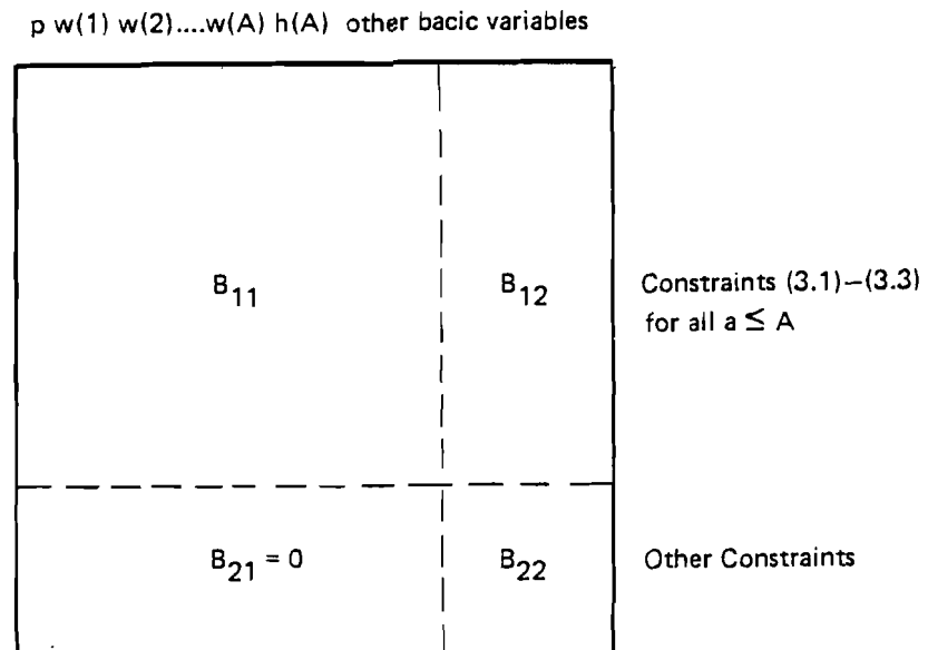
Figure: An optimal basis matrix for (F).
