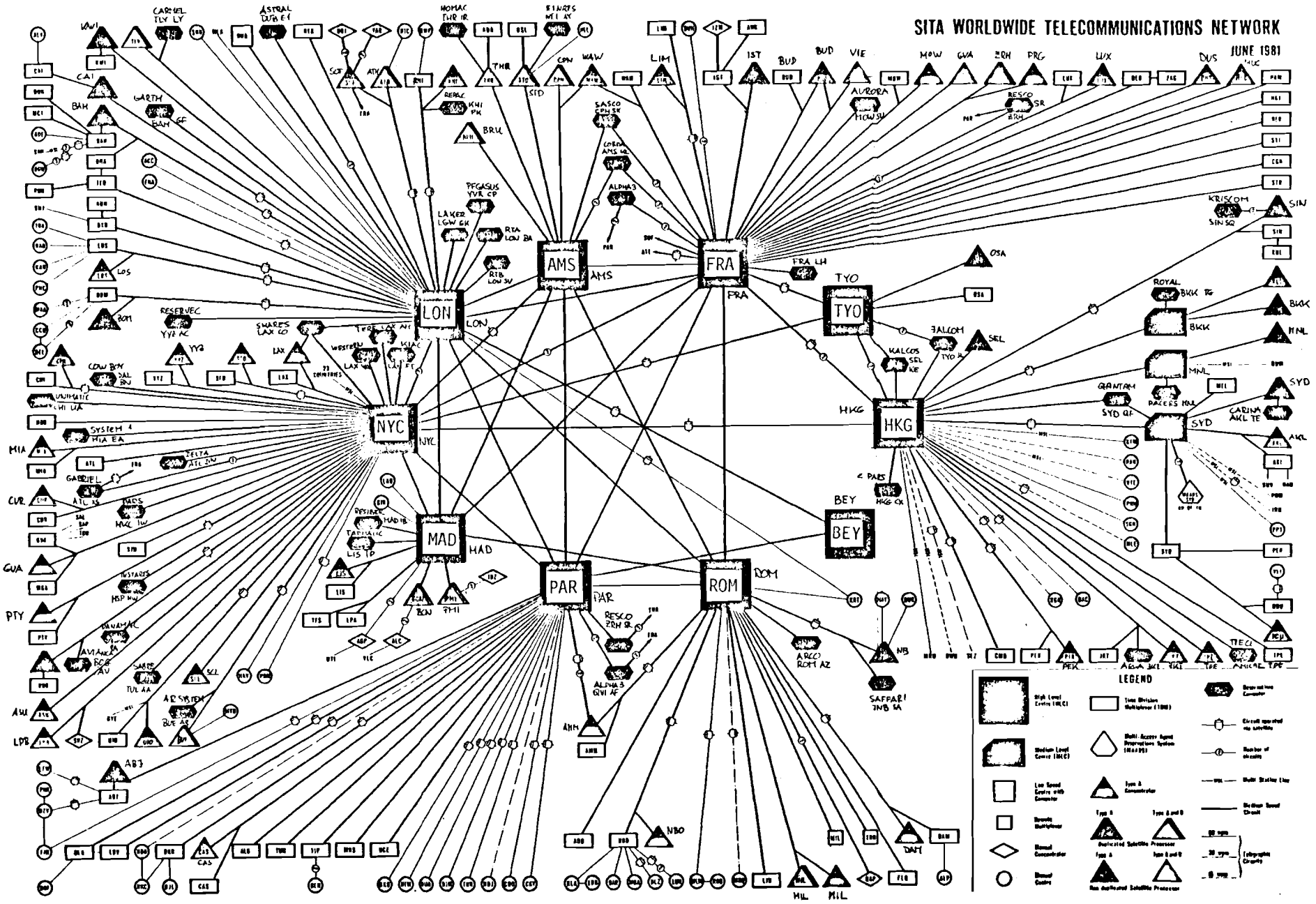
Figure 1. SITA worldwide telecommunications network.
