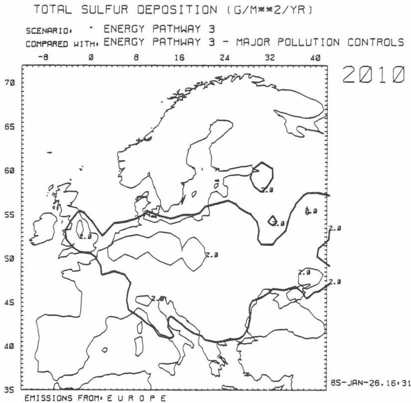
Figure 11. Computed sulfur deposition in Europe for the two scenarios in Figure 10. Computed location of the line of 2\text{ g m}^{-2}\text{ year}^{-1} total sulfur deposition: ---, energy pathway three without pollution controls; . . . ., energy pathway three with "major pollution controls".
