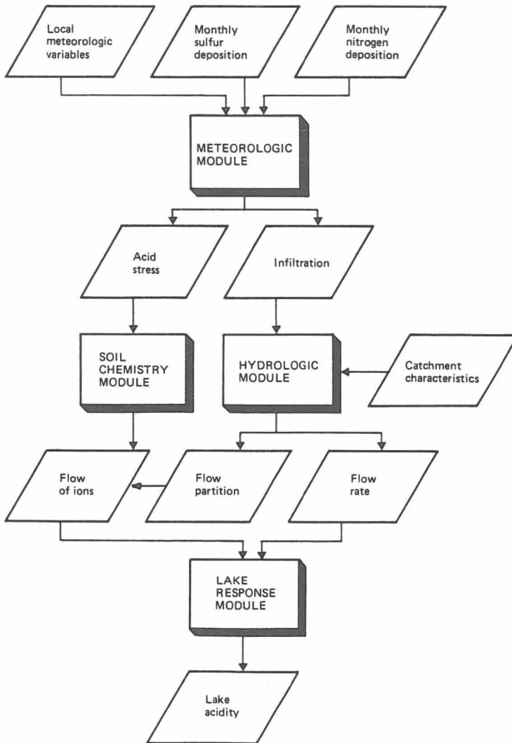
Figure 5. Sequence of calculations in Lake Acidity submodel.
