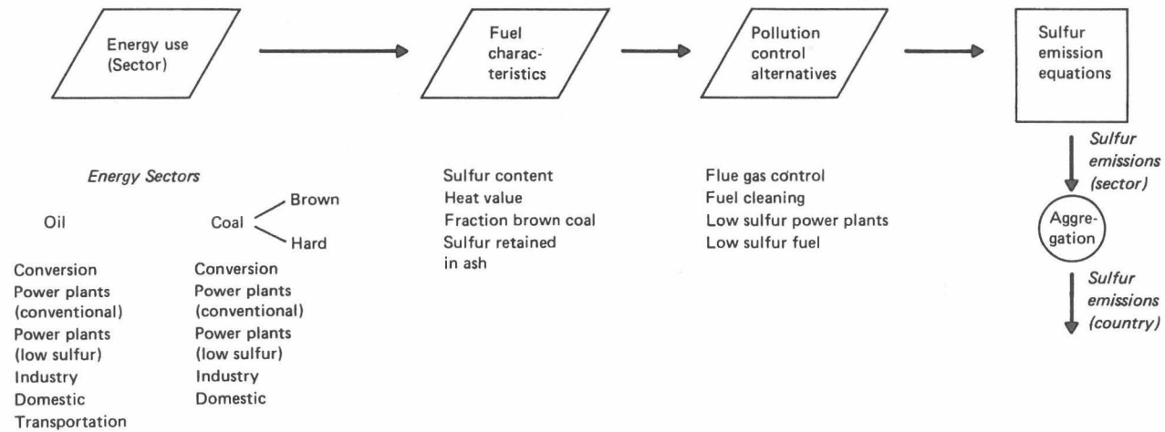
Figure 2. Sequence of calculations in Sulfur Emissions submodel.
