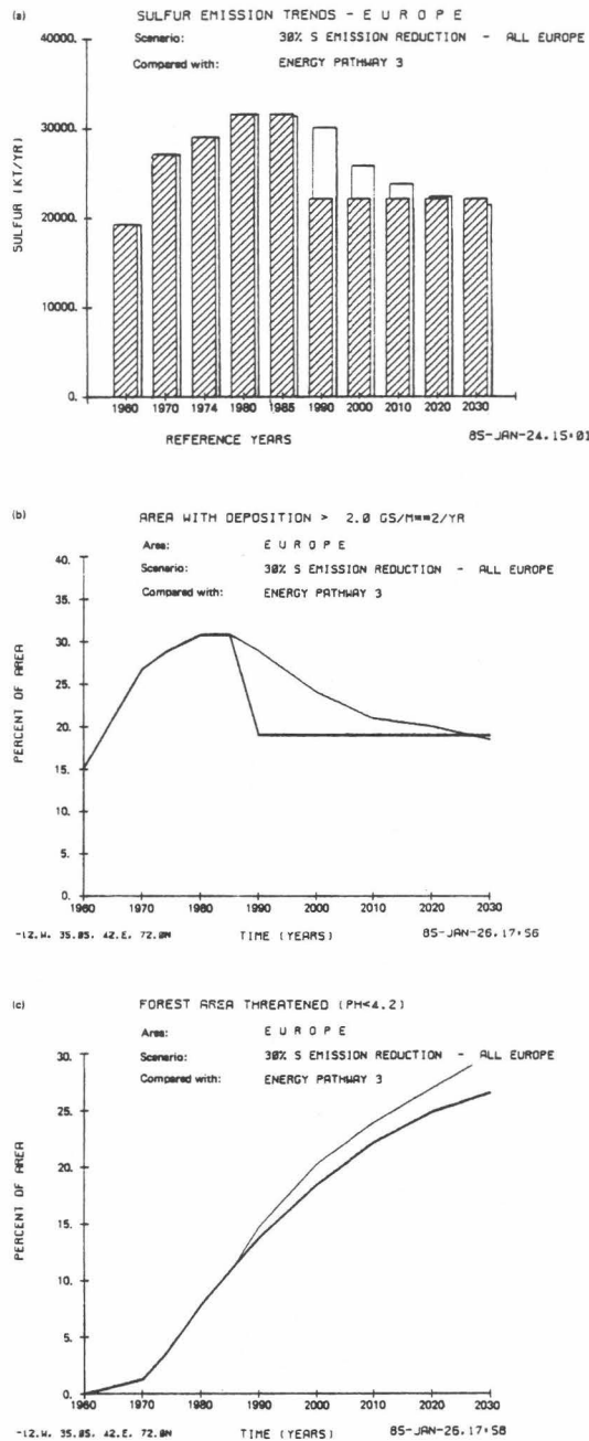
Figure 8(a). The total European sulfur emissions for both scenarios. The lined bars refer to the scenario of 30% sulfur emissions reduction while the open bars refer to the scenario of energy pathway number three. Note that sulfur emissions of both scenarios are roughly equal after the year 2020. (b) The area of Europe covered by \geq 2.0 \text{ g m}^{-2} \text{ year}^{-1} of sulfur deposition for the two scenarios. The heavier line refers to 30% sulfur emission reductions and the lighter line to energy pathway number three. (c) The computed "forest area threatened" in Europe, as defined by soil pH < 4.2. The heavier line refers to the scenario of 30% sulfur emissions reduction and the lighter line to the scenario of energy pathway number three.
