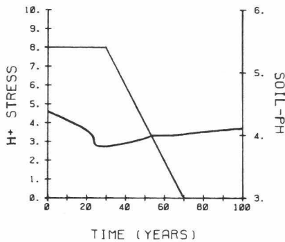
Fig. 3. Input-output relationship: response of the soil to a declining stress (thick line = soil pH).
