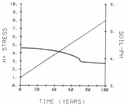
Fig. 2. Input-output relationship: response of the soil to an increasing stress (thick line = soil pH).
