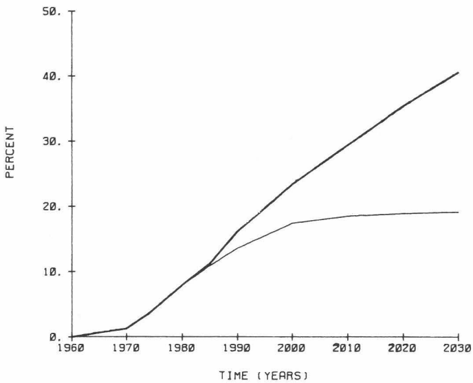
Fig. 8. Time evolution of the total forest area with soils in aluminium and iron buffer range (pH less than 4.2) in Europe assuming the two emission scenarios.
