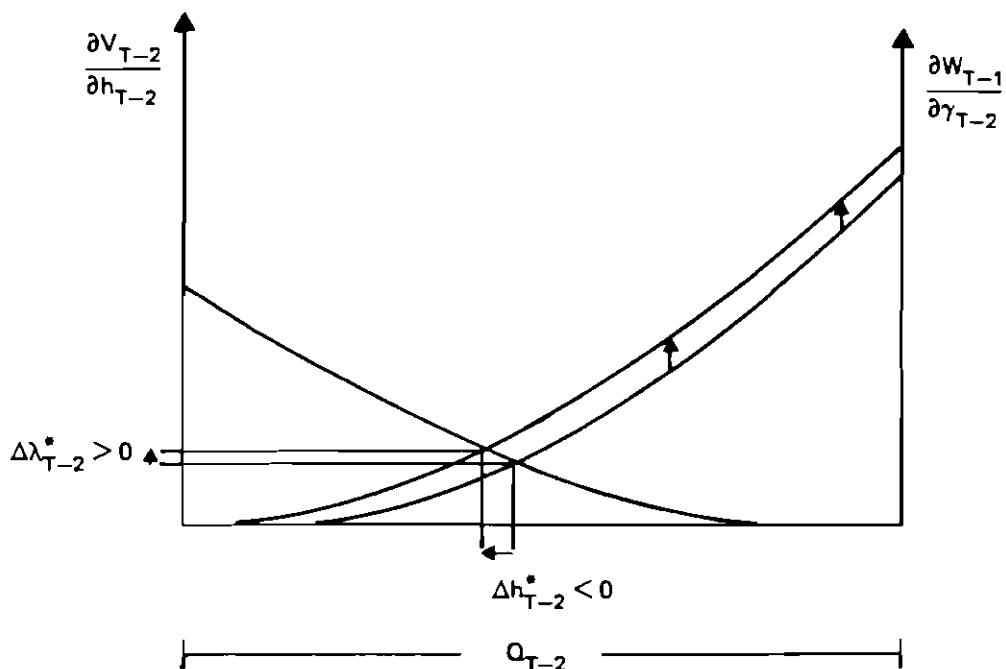
Figure 5.3 b In figure 5.3 a we obtained an increase in E_{T-2}^*(\lambda_{T-1}^*) .
