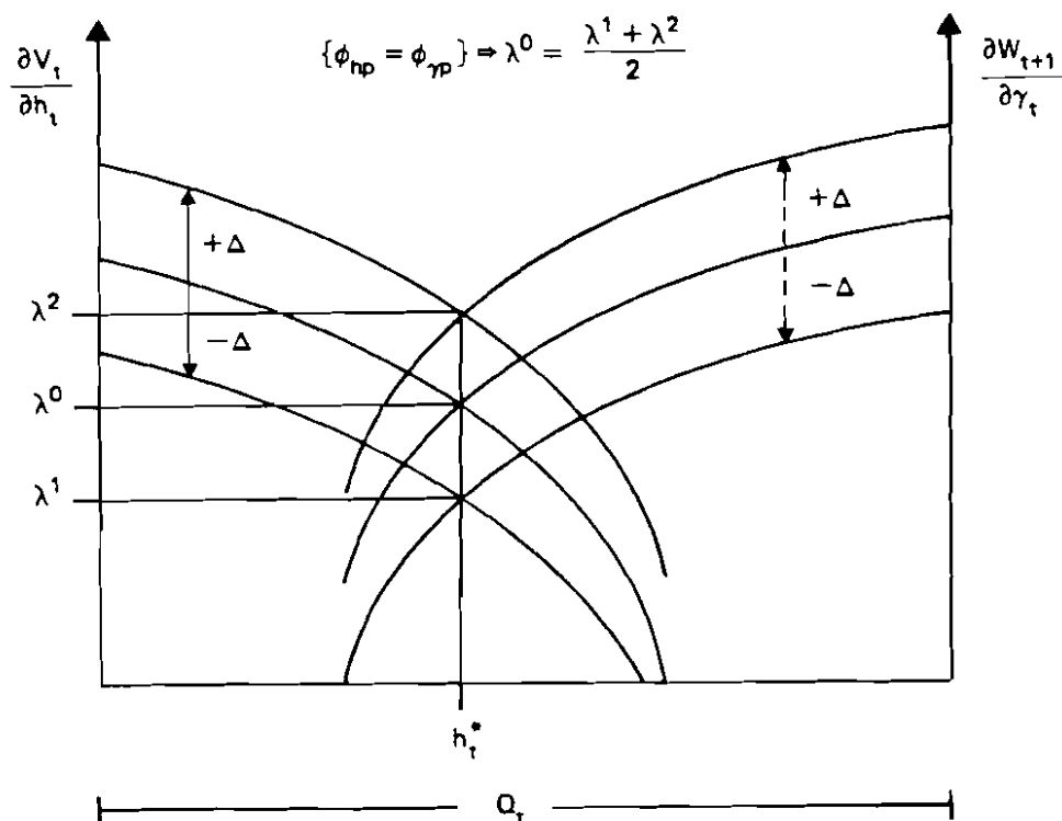
Figure 5.4 Let us assume that \phi_{hp} = \phi_{\psi p} . A change in the price in period t will then not affect the optimal harvest level since the expected marginal profit from the saved resource changes equally much. This, in turn, implies that E_{t-1}(\lambda_t^*) is unaffected by increasing risk in P_t , and h_{t-n}^* ( n > 1 ) will not change. (See remark 3.)
