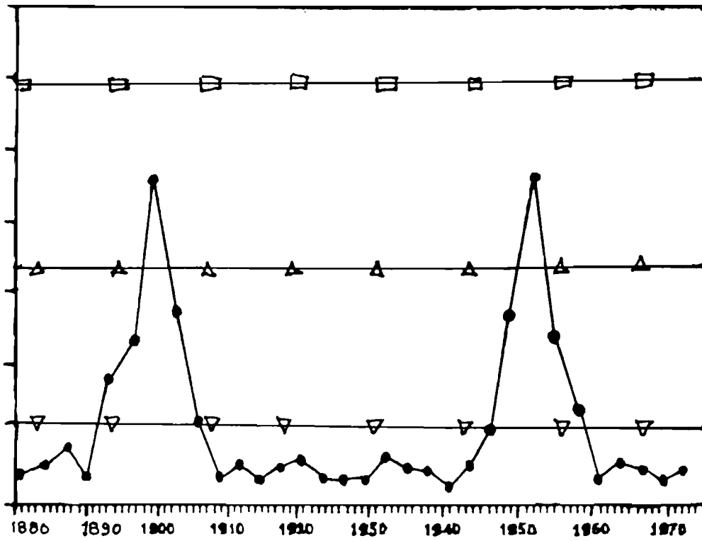
Figure 7: A pattern produced by an invalid measure
