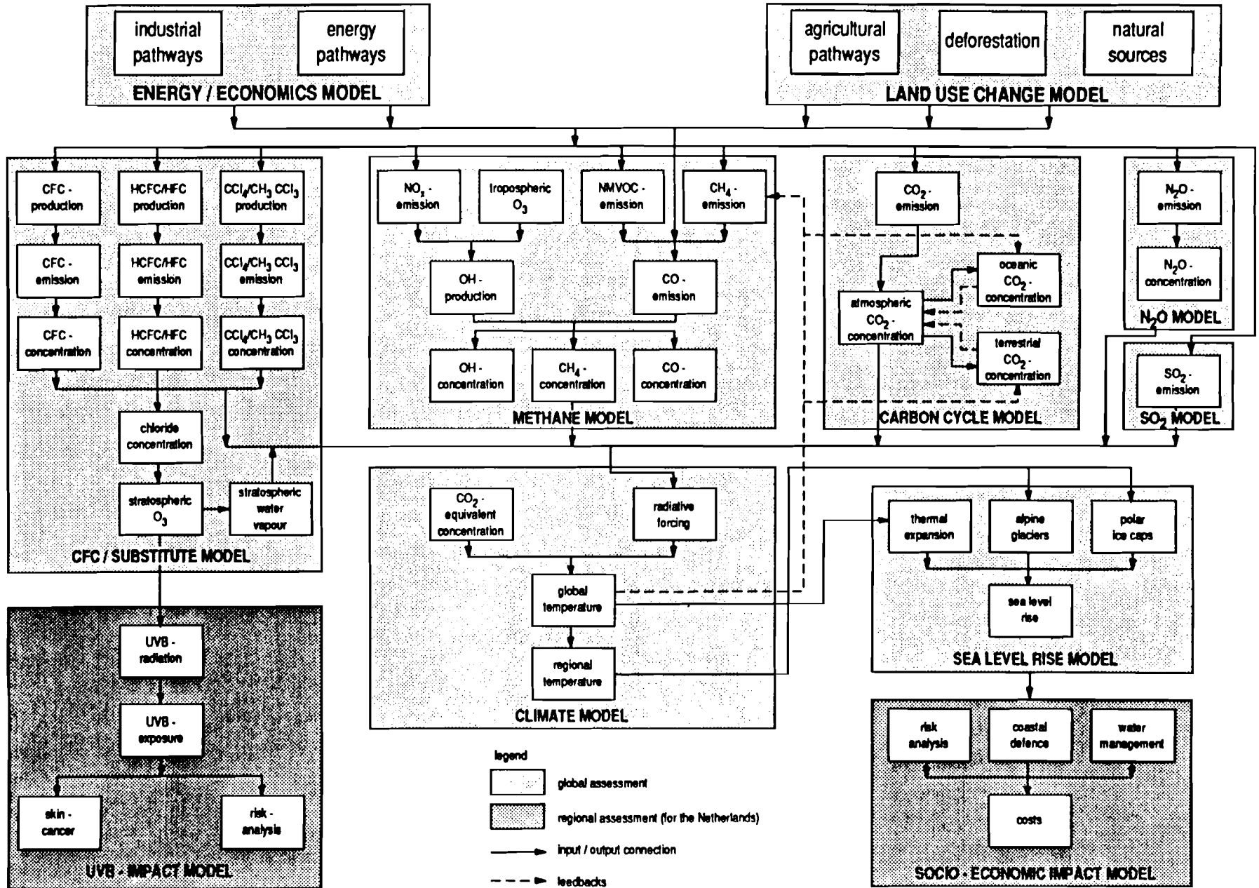
Figure 4: Detailed structure of IMAGE (Rotmans et al., 1991).
