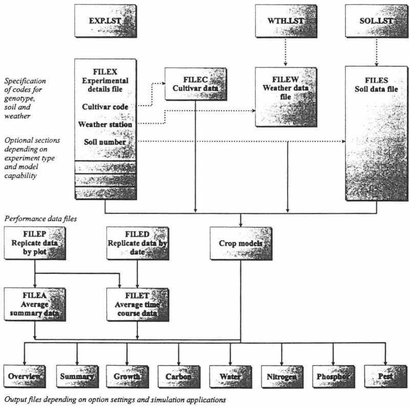
Fig. 2. The IBSNAT crop models.
