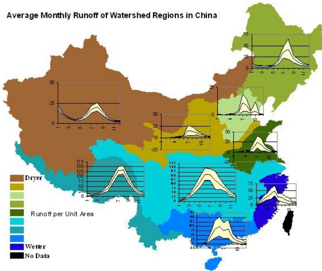
Figure 17: Map of the results of CHARM simulation for nine watershed regions over years 1965-1980. Each line on the charts represents 25 billion cubic meters. One standard deviation is plotted to either side of the mean monthly value.
