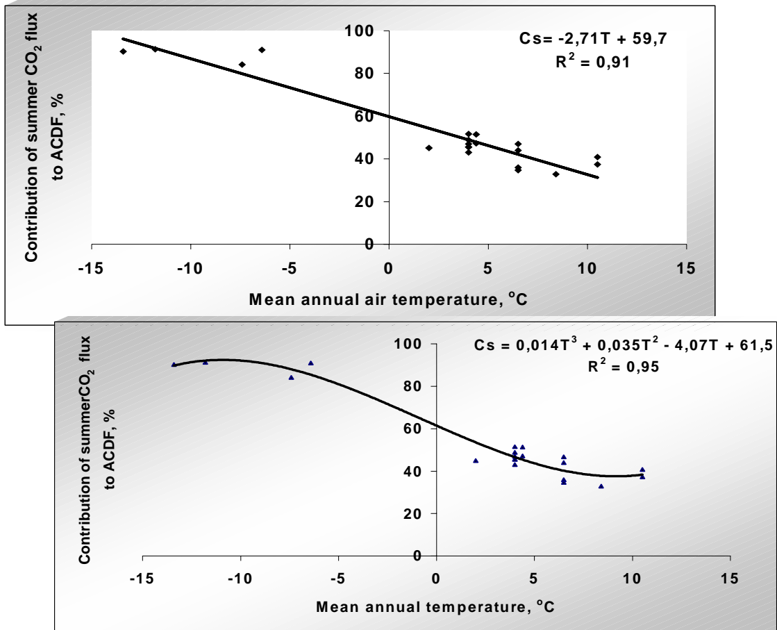
Figure 8: Linear and polynomial models for calculating summer CO_2 flux contribution to the annual flux.
