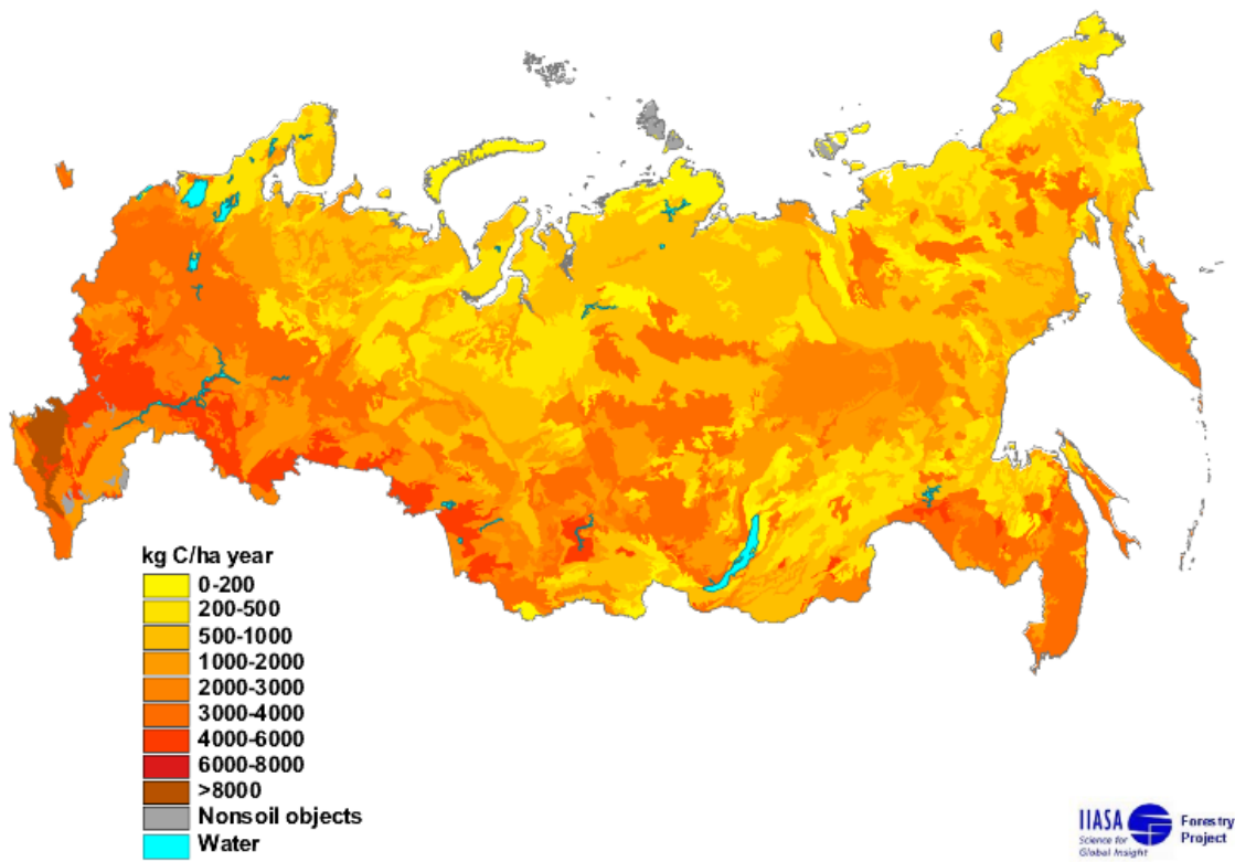
Figure 11: Heterotrophic respiration of Russian soils.
