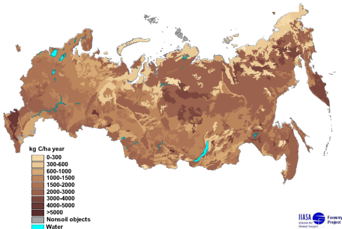
Figure 12: Root respiration of Russian soils.
