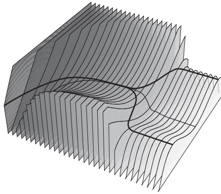
Figure 1 Adaptive speciation unfolding. A fitness landscape’s shape changes jointly with a population’s mean trait value (thick curve; the initial snapshot of the landscape is colored dark gray and the final one white). While the population undergoes directional selection by ascending the fitness landscape, the landscape itself changes because of frequency-dependent selection in such a way that a fitness minimum (thin curve) catches up with the population. Once trapped at the minimum, the population experiences disruptive selection and (under certain conditions) splits into two branches. In the figure, this divergence continues until the two branches arrive at local fitness maxima, at which selection becomes stabilizing.
