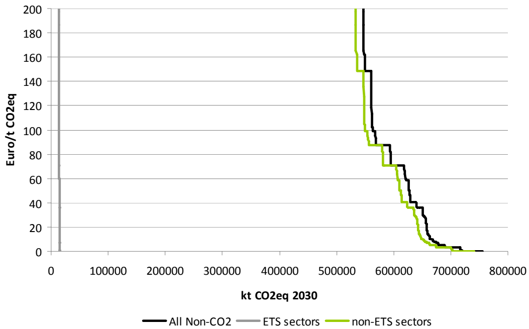
Figure 6: Marginal mitigation cost curve for non-CO 2 GHG in EU-27 2030, in total and split by ETS and non-ETS sectors.
