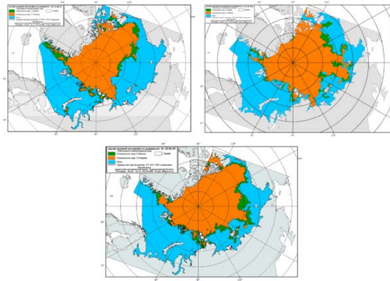
Figure 21 Ice area in the Arctic Ocean in August of 2007–2009.
