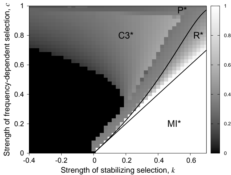
Figure 5: Frequency of the intermediate phenotype in the two-locus model, when simulations are started from random mating. Shades of gray indicate the frequency of the phenotype x = 0 , ranging from 0 (black) to 1 (white). The upper continuous line shows the border between the R^* and P^* domains, while the lower continuous line shows the border between the R^* and the MI^* domains. Across the R^* domain, the frequency of the intermediate phenotype increases from 0.5 (at the boundary to the P^* domain) to 1 (at the boundary to the MI^* domain). This is achieved by an increasing asymmetry of the allele frequencies at the ecological loci, 0.5 \pm \alpha , with \alpha increasing from 0 to 0.5.
