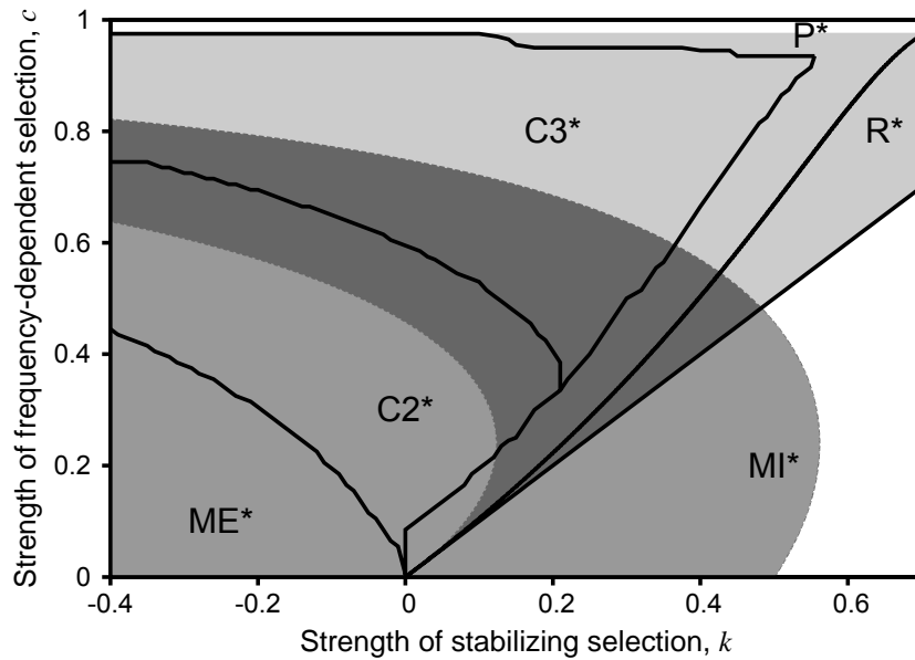
Figure 3: Evolutionary regimes for the model with two diallelic ecological loci of equal effect. Continuous lines and labels with asterisks indicate domains, in which different evolutionary equilibria are reached when simulations start from random mating ( m = 0 ). C2*: two species; C3*: three species; P*: partial isolation; R*: random mating; ME*: monomorphic equilibrium with extreme phenotype; MI*: monomorphic equilibrium with intermediate phenotype. Shades of gray show the local stability of complete-isolation equilibria with either two or three species, as determined from simulations started at m = 1^- = 0.999999 . In the light gray area, only the three-species equilibrium is locally stable. In the medium gray area, only the two-species equilibrium is locally stable. In the dark gray area, both the two- and the three-species equilibria are locally stable. Simulations started with three species in the area in which only two species are locally stable reach the intermediate monomorphic equilibrium in the part overlapping with the MI* domain and the two-species equilibrium otherwise. The boundaries of the medium gray and dark gray areas are derived analytically as described in Appendix B. In particular, the upper boundary (local stability of two species) is identical to the corresponding line in Figure 1 and is, indeed, independent of the genetic architecture of the ecological trait.
