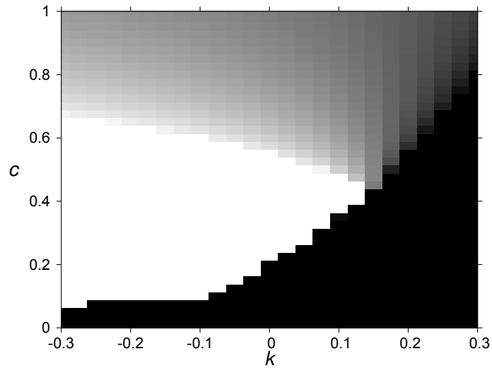
Figure A2: Evolution of assortative mating in the single-locus model with absolute viability costs and a single large mutational step (see Fig. A1 for more details). Shades of gray indicate the equilibrium frequency (black: 0, white: 1) of an “isolation allele” with m = 1^{-00.99} introduced at the low frequency p = 10^{-4} into a randomly mating resident population with m_r = 0 . The figure shows simulation results for the linear cost function (C.3) with \delta = 0.01 and \delta' = 0 . Note that, with this costs function, evolution of complete isolation through infinitesimally small mutational steps is always impossible.
