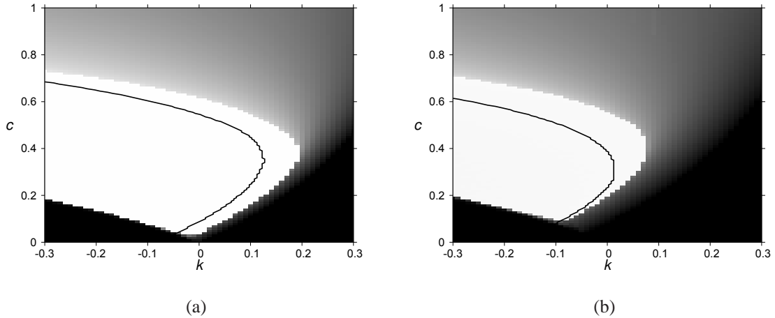
Figure A1: Evolution of assortative mating in the single-locus model with mating costs, assuming a single large mutational step. The number of mating trials per female is T = 10 in (a) and T = 5 in (b). Shades of gray indicate the equilibrium frequency (black: 0, white: 1) of an “isolation allele” with m = 1^- = 0.99 introduced at the low frequency p=10^{-4} into a randomly mating resident population with m_r = 0 . The continuous lines show the corresponding boundaries of the complete-isolation regime for infinitesimally small steps (calculated as in Kopp and Hermisson, 2008).
