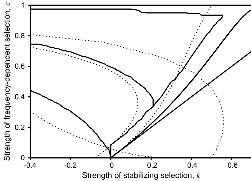
Figure 4: Comparison of the one- and two-locus models. The continuous lines are the domain boundaries for the two-locus model (delineating the outcomes from random mating), as shown in Fig. 3. The dashed lines are the domain boundaries for the one-locus model, as shown in Fig. 1.
