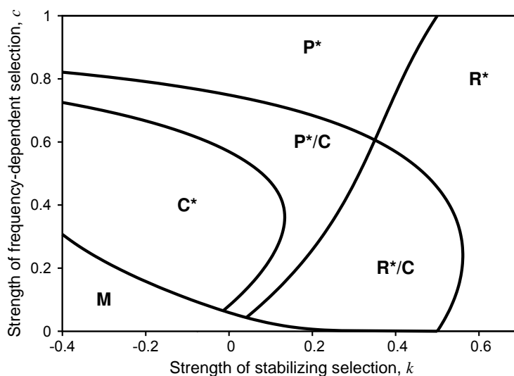
Figure 1: Evolutionary regimes in the baseline model. The ecological trait is determined by a single locus, and choosiness evolves in infinitesimal steps. Note that negative k implies that selection due to the carrying capacity function is disruptive. C*: complete isolation; R*: random mating; P*: partial isolation; R*/C: random mating or complete isolation; P*/C: partial or complete isolation; M: monomorphic outcome with only one extreme phenotype. The asterisk indicates that the outcome is reached from random mating. The boundary for the local stability of random mating and complete isolation is calculated according to Appendix A. The boundary of the C* regime is calculated numerically using equation (11), and the boundary of the M regime is determined by numerical stability analysis as in Pennings et al. (2008).
